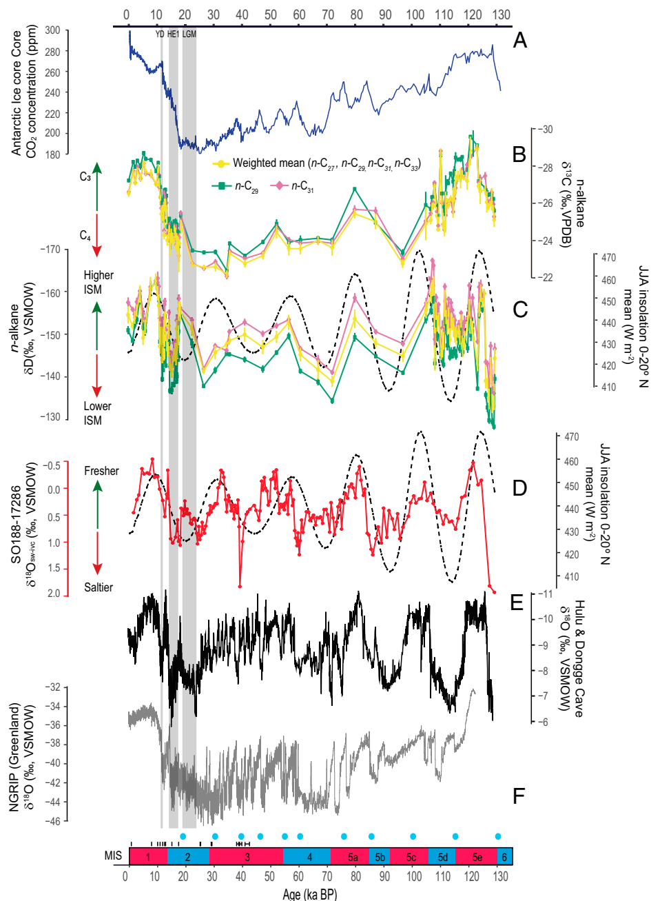
Fig. 2. Climate records derived from sediment core 17286-1 in comparison with other high- and low-latitude climate proxy records: (A) Antarctic ice cores composite CO 2 concentration (53, 54). (B) \delta^{13}\text{C} (mean \pm SE) of n\text{-C}_{29} and n\text{-C}_{31} and concentration-weighted average \delta^{13}\text{C} based on all four homologs ( n\text{-C}_{27} , n\text{-C}_{29} , n\text{-C}_{31} , and n\text{-C}_{33} ) from sediment core 17286-1 as a proxy for vegetation ( \text{C}_3 vs. \text{C}_4 plants) changes (this study). (C) Ice volume-corrected \delta\text{D} (mean \pm SE) of n\text{-C}_{29} and n\text{-C}_{31} and concentration-weighted average \delta\text{D}_{\text{ivc}} based on all four homologs ( n\text{-C}_{27} , n\text{-C}_{29} , n\text{-C}_{31} , and n\text{-C}_{33} ) from sediment core 17286-1 as a proxy for rainfall amount (this study). The dashed black line represents summer (JJA) mean insolation at 0 to 20°N (55). (D) Ice volume-corrected planktonic foraminiferal \delta^{18}\text{O} ( \delta^{18}\text{O}_{\text{sw-ivc}} ; red) as a proxy for local sea water salinity compared to boreal summer insolation as in Fig. 2C (27). (E) \delta^{18}\text{O} record from Chinese stalagmites (56), reflecting past EASM changes. (F) North Greenland Ice Core Project (NGRIP) ice core \delta^{18}\text{O} record (57), reflecting climate variability and particular Heinrich events in the Northern Atlantic realm. Gray bars mark the YD, HE1, and the LGM as reflected in the NGRIP ice core \delta^{18}\text{O} record as well as their correlatives in the Asian monsoon proxy records. Age control points for sediment core 17286-1 are also indicated, including radiocarbon dates (black lines) and tie points (blue circles) derived from tuning of the benthic foraminifera \delta^{18}\text{O} record to the LS16 global \delta^{18}\text{O}_{\text{benthic}} stack (47). Red and blue intervals at the bottom delineate MISs, separating warm and cold climate periods, respectively.
