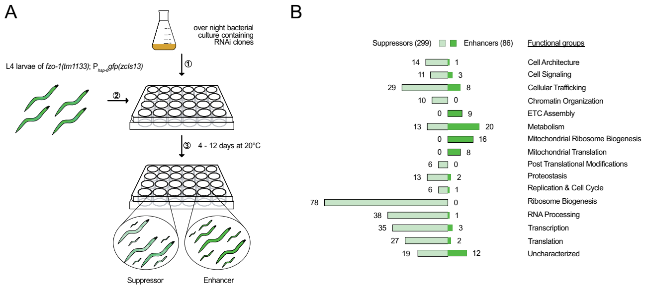
Figure 1 Overview of genome-wide RNAi screen for suppressors and enhancers of fzo-1(tm1133) -induced UPR^{mt} . (A) Schematic overview of the RNAi screening procedure using the RNAi feeding library (Kamath and Ahringer 2003) in fzo-1(tm1133) mutants that express the UPR^{mt} reporter P_{hsp-6} mtHSP70gfp ( zcls13 ). The moderate induction of the reporter in the fzo-1(tm1133) background allowed screening for both suppressors and enhancers of the response. (B) The screen resulted in identification of 299 suppressors and 86 enhancers of fzo-1(tm1133) -induced UPR^{mt} , which were sorted into categories that we defined according to their function. ETC, electron transport chain.
