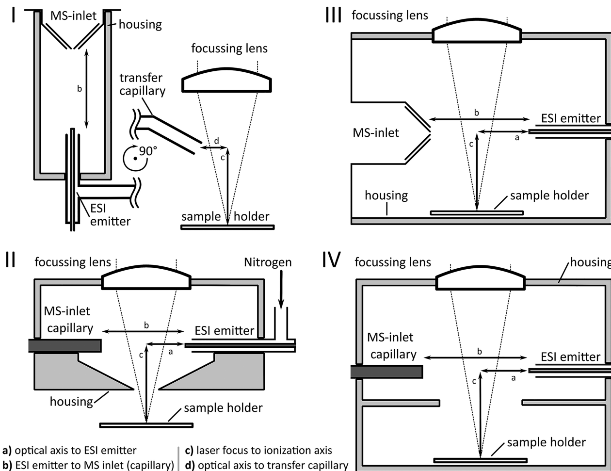
Figure 1. Schematic representations of the investigated LAESI ion source geometries, namely, coaxial ionization (I), the ionization chamber (II), and classic LAESI geometries (III), as well as the commercial DP-1000 LAESI ion source (IV).
