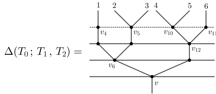
Figure 13: The leveled tree \Delta(T_0, \{T_i\}) associated to the family represented in Figure 11.
