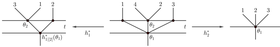
Figure 18: Illustrations of the \Lambda -structure associated to h_1, h_2 : [3] \rightarrow [4] with h_1(i) = i + 1 and h_2(i) = i .
