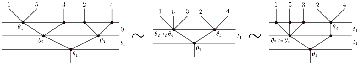
Figure 17: Illustration of equivalent points in W_l\mathcal{O}(5) .
