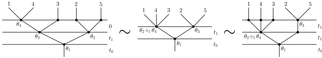
Figure 16: Illustration of equivalent points in \mathcal{B}_l(\mathcal{O})(5) .
