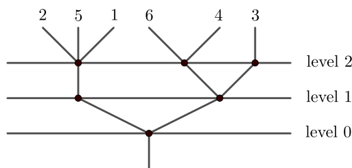
Figure 2: A leveled 6-tree.
