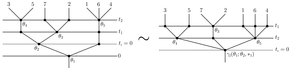
Figure 20: Illustration of equivalent points in W_l M(7) .
