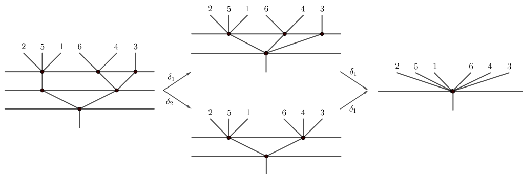
Figure 3: Contraction morphisms in the category \mathbb{L}[6] .
