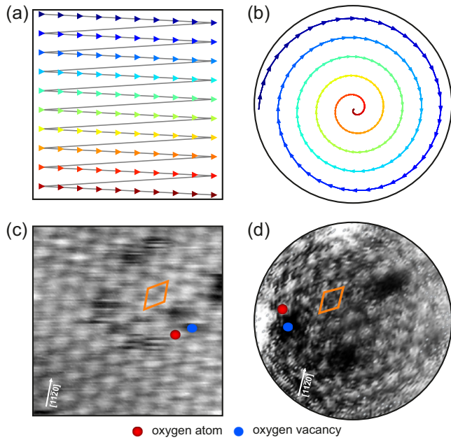
FIG. 2. Raster and spiral scan STM images. (a) Schematic raster scan trajectory. The triangular shaped data points indicate a forward downward scan. (b) Schematic spiral scan trajectory of an Archimedean spiral at CAV. The triangles indicate the inward scan direction. The data point density in the center is increased due to the lower linear velocity of the tip. (c) and (d) Atomically resolved STM images of the O(2 \times 2) layer on Ru(0001) ( V_s = 1 V, I_T = 1.4 nA, T = 300 K). (c) Raster scan STM image acquired in constant current mode in 100 s (scan area = 5 nm \times 5 nm). (d) High-speed spiral scan STM image acquired in quasiconstant height mode in 50 ms (scan diameter = 5 nm). Oxygen and oxygen vacancy positions are marked exemplarily. The unit cell is drawn in orange.
