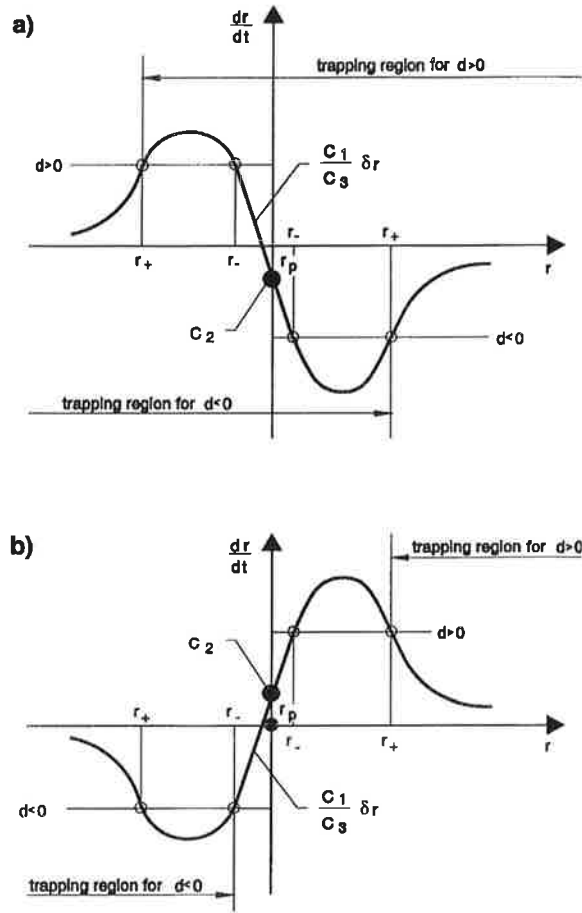
Figure 3.3: Orbit trapping in resonant potential canyon (panel a) and at potential energy barrier (panel b)
