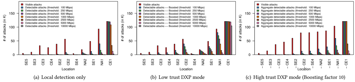
Figure 19: Absolute: Detectable DDoS attacks for low and high trust DXP vs. local detection at a single IXP without DXP.
