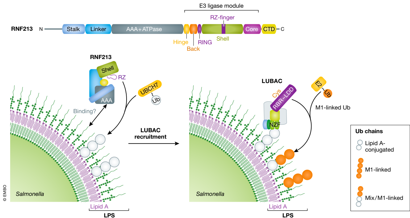
Figure 5. The atypical E3 ligase RNF213 ubiquitylates LPS on Salmonella .
