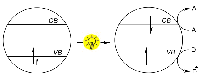
Figure 1.9. Charge separation in semiconductors upon light absorption.
