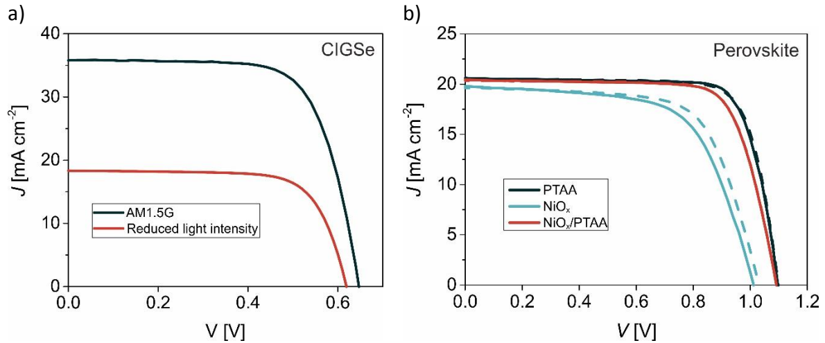
Figure 4: J-V characteristics of a) CIGSe single-junction reference under AM1.5G and reduced light intensity and b) perovskite single-junction reference cell with different HTLs: PTAA (black), NiO x (blue) and NiO x /PTAA (red) under AM1.5G. Solid lines show forward ( J_{sc} to V_{oc} ) scan and dashed lines reverse ( V_{oc} to J_{sc} ) scan direction. The performance parameters are stated in Table 1.
