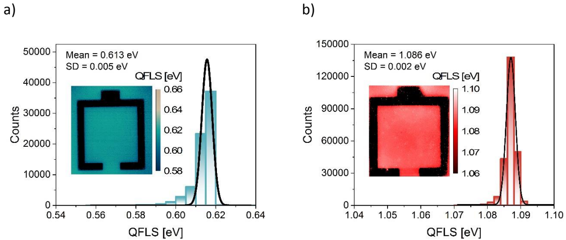
Figure 5: Quasi-Fermi level splitting (QFLS) maps and histogram obtained from absolute PL mapping of the perovskite/CIGSe tandem device: a) CIGSe bottom cell and b) perovskite top cell. From the histogram, the QFLS of 0.613 eV for CIGSe and b) 1.086 eV for the perovskite can be estimated.
