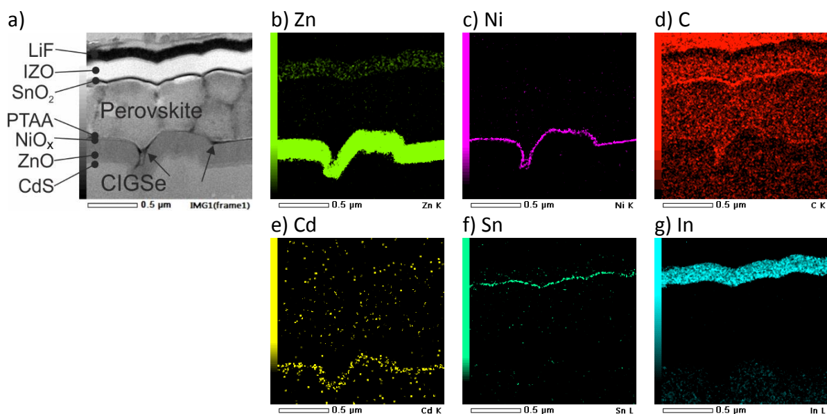
Figure 2: Cross sectional HAADF-STEM images (a) and elemental maps (b-g) deduced from EDX measurements of the fabricated tandem device with a focus on the perovskite top cell. a) STEM of a peak-valley-shaped region, where depletion and agglomeration of PTAA is visible (see arrows), confirmed by an increased carbon signal in the EDX image d). Ni (violet) on the other hand covers both the valley and the peak conformally. Zinc is depicted by green, Ni violet, carbon (PTAA) red, cadmium yellow, tin turquoise and indium cyan color.
