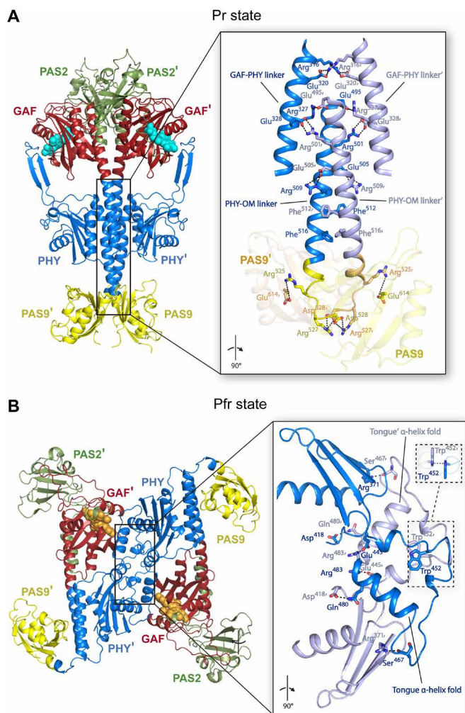
Fig. 7. The XccBphP full-length Pr and Pfr structures reveal different quaternary arrangements. (A) Head-to-head dimer assembly of the wild-type Pr crystal structure as found in its asymmetric unit. (B) Head-to-tail crystallographic dimer assembly of the G454E Pfr crystal structure constructed by means of the -x, -y, z symmetry operator of the I4_1 space group. (A and B) Structures are shown in ribbon representation and colored following Fig. 3 domain color code with the two protomers depicted in different shades. Insets: Detailed view (rotated 90^\circ with respect to main panels) of the respective dimerization interfaces encompassing the GAF-PHY and PHY-OM helical linkers from the helical spine in the Pr structure and the tongue region in the Pfr structure. Interfacing residues are depicted as sticks and colored according to their corresponding chain. Important polar interactions are shown as black dashed lines. Two views of the \pi - \pi stacking interaction between Trp 452 /Trp 452' (from the Trp switch) in the Pfr structure are enclosed in dashed boxes.
