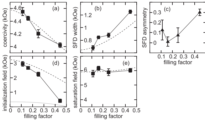
FIG. 3. Parameters resulting from fitting the hysteresis loops presented in Fig. 2: (a) coercive field ( H_C ), (b) width of the SFD ( \sigma ), and (c) asymmetry ( \alpha ). (d) Initialization fields and (e) saturation fields as extracted from the same fits. The error bars were obtained from the uncertainty of the fits of the hysteresis loops. The dashed and dotted lines are calculations according to an analytical magnetostatic model as explained in the text.
