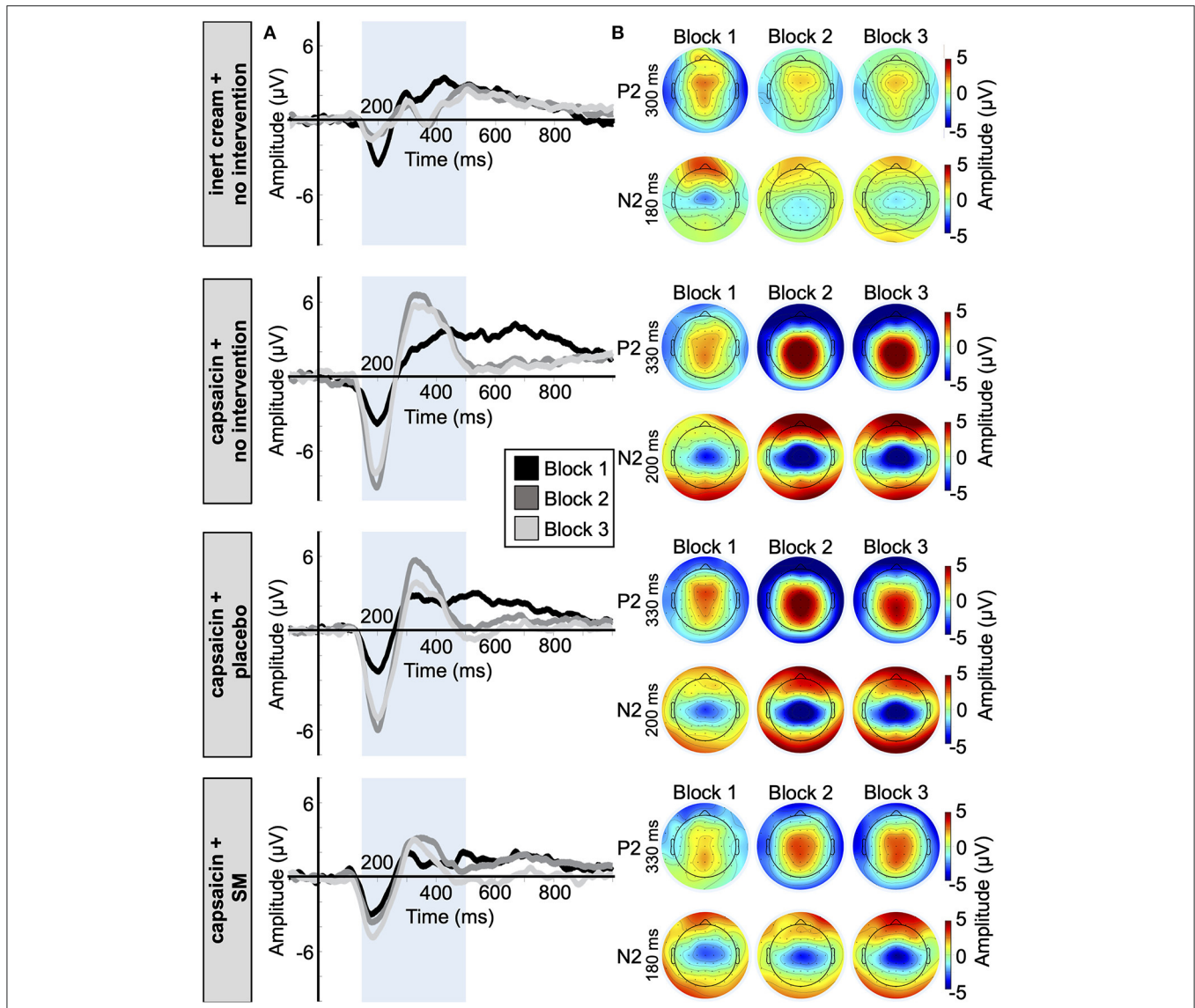
FIGURE 6 | A \delta fiber laser-evoked potentials. (A) Average waveforms for the N2 and P2 at Cz with a nose reference of the 77 participants included in the A \delta fiber LEP analysis, time-locked to the onset of laser stimulation. (B) Average topographic maps for the A \delta -N2 and A \delta -P2 in the four groups.
