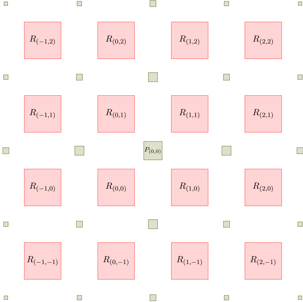
FIGURE 2.6: The cubes R_m (in red) and P_m (in green) in \mathbb{R}^2 , with m = (m_1, m_2) , for \ell_m = \frac{1}{|m|+1} . Each R_m has side length 2 and P_m has sidelength \ell_m .
