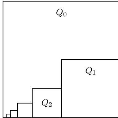
FIGURE 3.1: The cubes Q_j for j \geq 0 in dimension 2.
