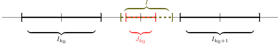
FIGURE 2.4: Case 2b: |I \cap A| = 0 , |I| > |J_{k_0}| .
