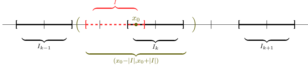
FIGURE 2.2: Case 1: |I \cap A| > 0 .
