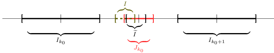
FIGURE 2.3: Case 2a: |I \cap A| = 0 , |I| \leq |J_{k_0}| .
