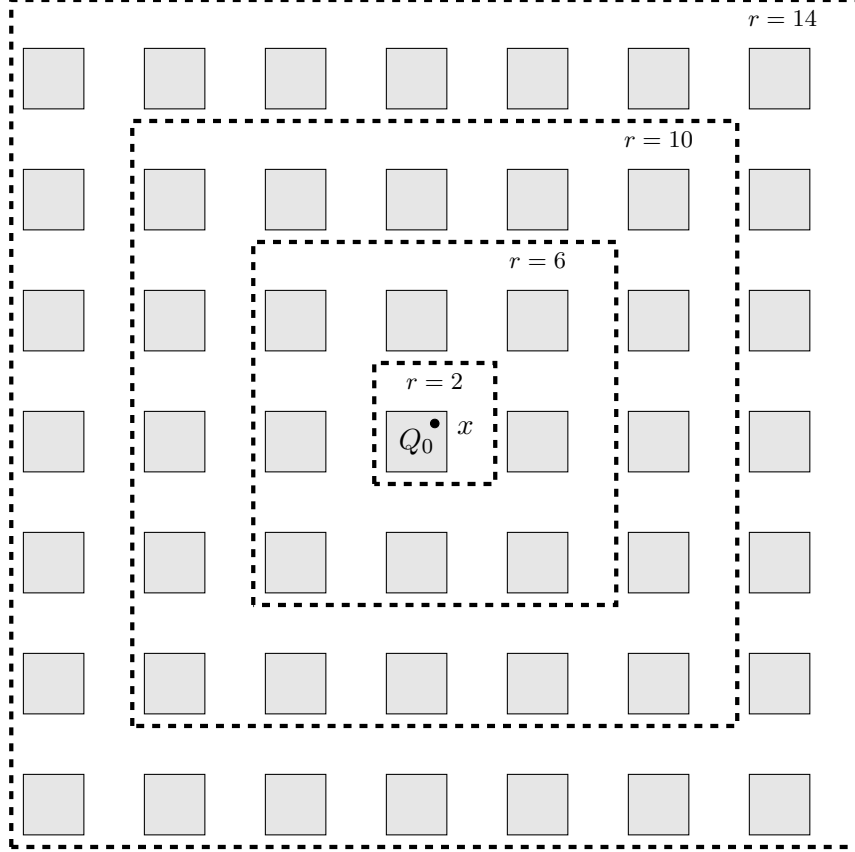
FIGURE 2.5: Scheme in dimension 2. Q_0 = [-1, -3]^2 and each of the grey cubes has sidelength 2, at distance 2 from each other. The dashed lines represent cubes centered at x with sidelength 2r , for the values r = 2, 6, 10, 14 .
