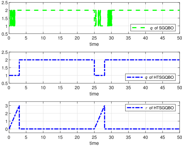
Fig. 11. Evolution of q given by the SGQBO and of q, \tau given by the HTSQBO.
