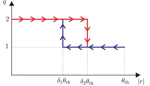
Fig. 1. Switching rule based on hysteresis.
