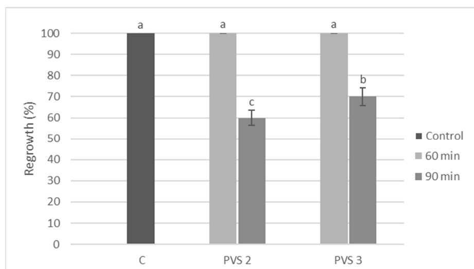
Figure 2. Effect of vitrification solutions (PVS2 or PVS3), applied for 60 or 90 min, on regrowth (%) of axillary buds of Corylus avellana , cultivated variety Tonda Gentile Romana, not immersed in liquid nitrogen. Control (C) indicates explants directly transferred to the recovery solution after loading phase. Error bars indicate SE. Bars marked with the same letter are not significantly different according to Tukey's test ( p \leq 0.05 ).
