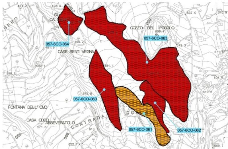
Figure 1. Hydrographic basin of Belice river (057) - excerpt of the Map of Instability n. 19, including the surveyed area: the areas where soil erosion caused landslides are highlighted, i.e. those having active landslides are in red colour, while those having landslides at rest are in yellow colour (Sicilian Region - Territory and Environment Department, Basin Shred Plan for Hydrogeological Layout, 2005).
