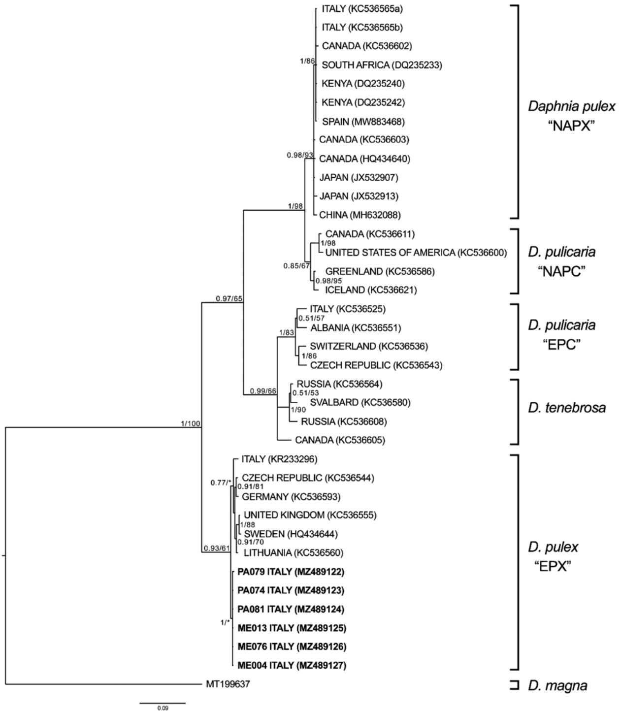
Fig. 2. Bayesian phylogram of Daphnia spp. based on the 624 bp fragment of the mtDNA ND5. D. magna was used as outgroup. Node statistical support is reported as nodal posterior probabilities (Bayesian Inference of phylogeny, BI)/bootstrap values (Maximum Likelihood, ML). *, Nodal statistical supports <0.50. Square brackets group the samples according to the current taxonomy of the genus. Novel sequences are reported in bold. NAPX, North American Pulex; NAPC, North American Pulicaria; EPX, European Pulex; EPC, European Pulicaria. The analysed specimens are reported using the codes listed in Tab. 1.
