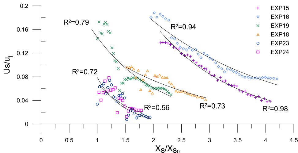
Fig. 8 Trend of the streamwise velocity along the jet trajectory, with fitting exponential curves
