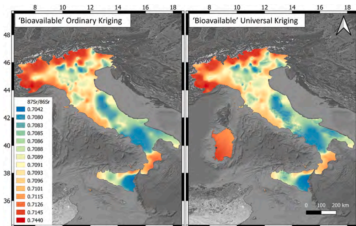
Fig. 4. Ordinary and Universal (with external drift) kriging models obtained for the ‘bioavailable’ ^{87}\text{Sr}/^{86}\text{Sr} dataset. Maps were obtained using SAGA 7.9 and QGIS 3.8.
