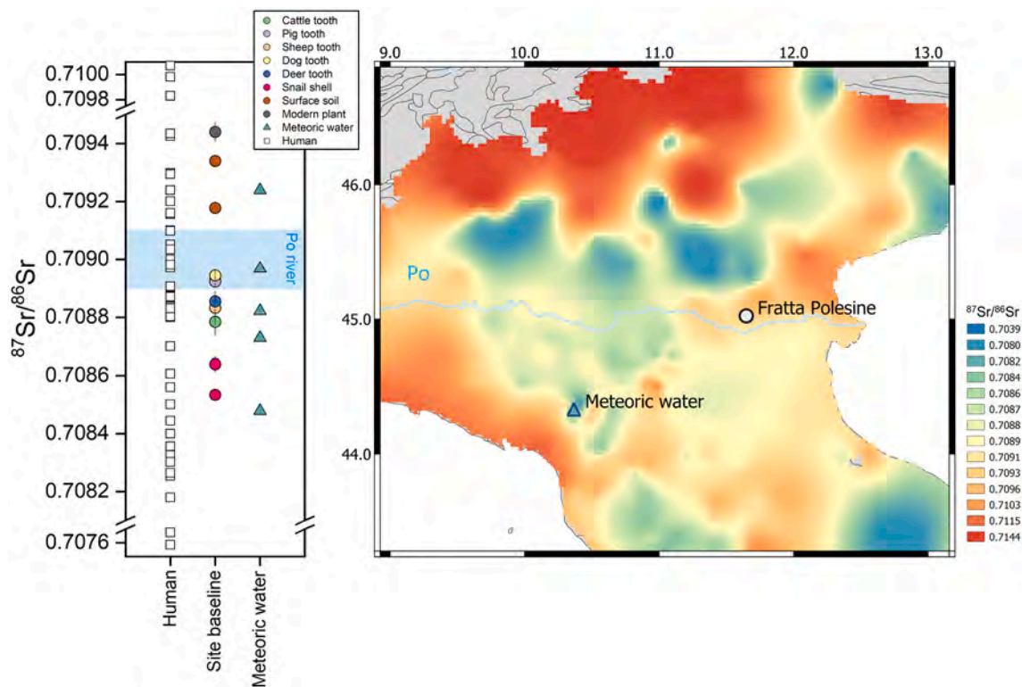
Fig. 6. Local baseline at the Bronze Age site of Fratta Polesine (Rovigo, Veneto). Analysed samples include animal tooth enamel, snail shells, surface soil leachates and vegetation. Human data (including both enamel and cremated petrous bone specimens) are from Cavazzuti et al. (2019a). In the graph, meteoric water data from the Apennines (blue triangles) and water data (light blue area) from the Po river (sampling locations close to the site) are reported for comparison. The Sr bioavailable map on the right panel is an Ordinary Kriging interpolation, without the local data from Fratta Polesine. The local (<10 km) predicted ^{87}\text{Sr}/^{86}\text{Sr} range at the site is 0.7091–0.7096 (median 0.7094). The Po river is also shown on the map. (For interpretation of the references to colour in this figure legend, the reader is referred to the web version of this article.)
