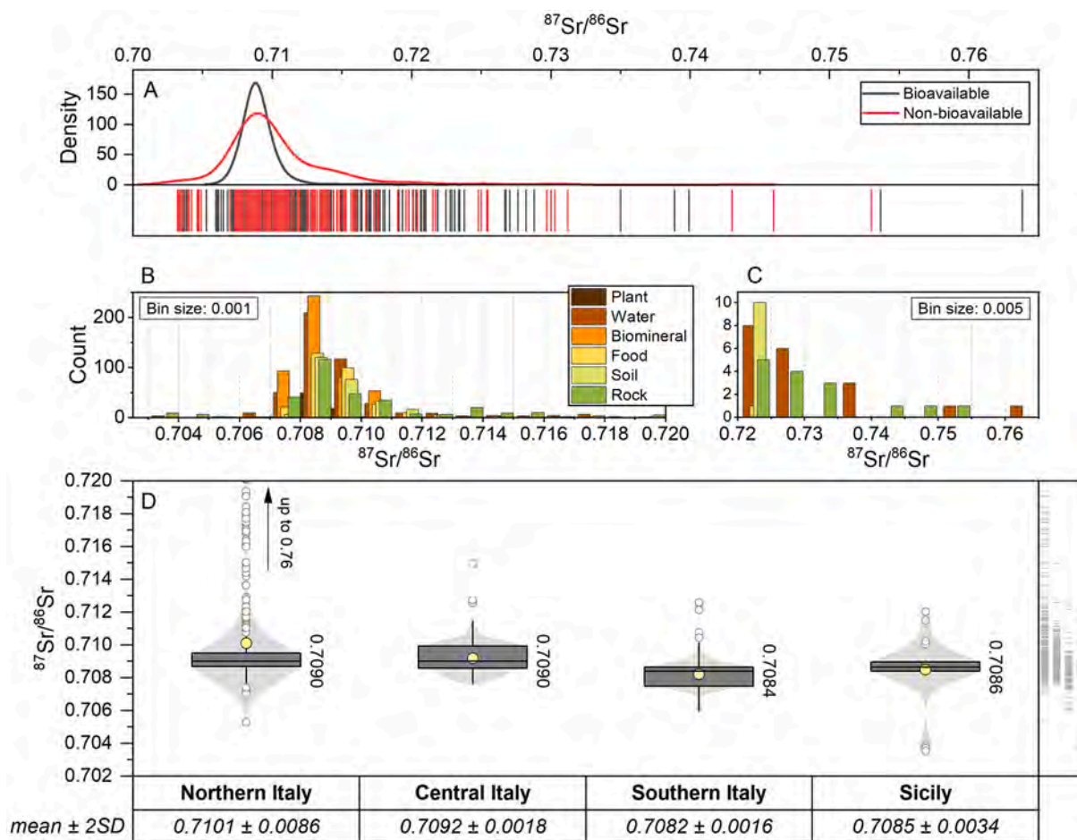
Fig. 2. Data exploration. A) Kernel density estimation of bioavailable (n = 1568) vs. non-bioavailable (n = 352) ^{87}\text{Sr}/^{86}\text{Sr} data. B) Superimposed histogram representing the different sample categories between 0.702 and 0.720, with a bin size of 0.001. C) Superimposed histogram of the different sample categories between 0.720 and 0.77, with a bin size of 0.005. Note that the y-scale ranges of the histograms ('count') are different. D) Bioavailable Sr isotope data grouped by geographical areas (macroregions) of Italy, defined according to the National Institute of Statistics (istat.it); median values are labelled close to the box plots; average values \pm 2 SD are also reported.
