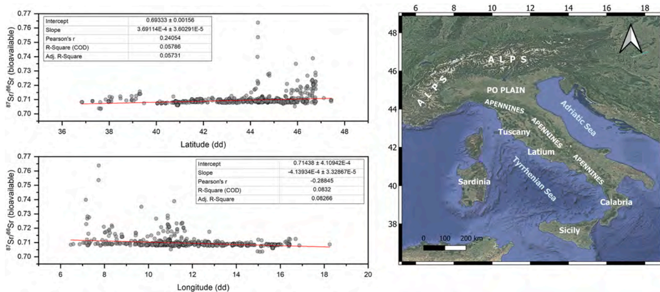
Fig. 3. The ^{87}\text{Sr}/^{86}\text{Sr} ratios plotted against latitude and longitude (decimal degrees). No significant linear trend appears; however, most of the radiogenic Sr data are latitudinally distributed northwards and longitudinally eastwards. Graphs and linear trends were produced using Origin v. 2020. Right panel: a geographic map of Italy is reported as reference; the main areas cited in the manuscript are labelled.
