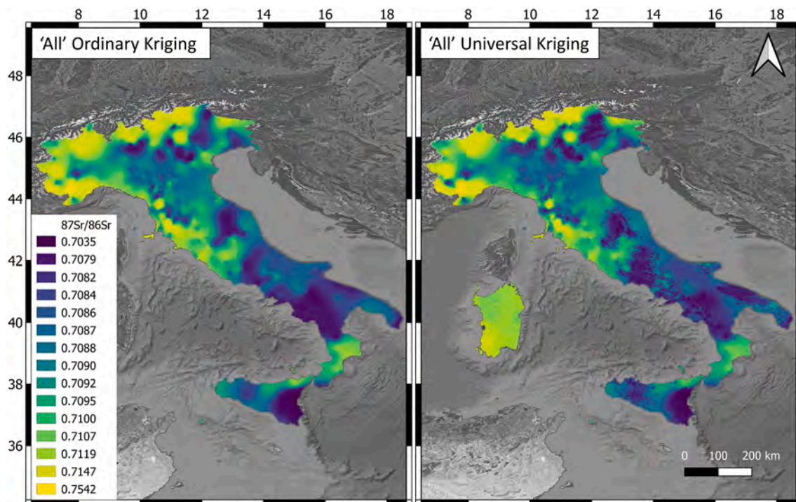
Fig. 5. Ordinary and Universal (with external drift) kriging models obtained for the 'all' ^{87}\text{Sr}/^{86}\text{Sr} dataset. Maps were obtained using SAGA 7.9 and QGIS 3.8.
