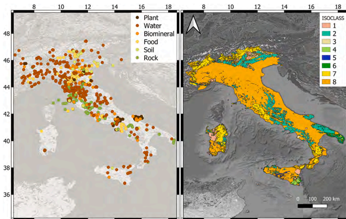
Fig. 1. Left panel: locations of the data points considered in this study. Most of the data are from literature, with the addition of novel unpublished environmental/archaeological samples. All the samples in the 'plant', 'water', 'biomineral' and 'food' categories are considered 'bioavailable', in addition to 'soil' leachates. 'Rock' and bulk 'soil' are considered 'non-bioavailable'. This map was built in QGIS 3.18.1 (QGIS Development Team 2021, QGIS Geographic Information System. Open Source Geospatial Foundation Project. http://qgis.osgeo.org ), exploiting the OpenStreetMap service. Right panel: Isoclass map of Italy that is a map of the Italian geolithologies classified according to their expected isotope values. This map is based on the geolithological map of Italy available at the Geoportale Nazionale ( http://wms.pcn.minambiente.it/ogc?map=/ms_ogc/wfs/Carta_geolitologica.map ); the satellite map is provided by Google through the QGIS QuickMapServices plug-in. Isoclass 1: plutonic and volcanic rocks related to MORB mantle magmatism of different ages. Isoclass 2: marine carbonate rock formations of Late Triassic, Cretaceous and Jurassic ages. Isoclass 3: Early and Middle Triassic and Paleogene marine carbonate rocks. Isoclass 4: Early and Medium Miocene marine carbonate formations. Isoclass 5: Late Miocene carbonates. Isoclass 6: Pleistocene and Pliocene carbonate formations. Isoclass 7: old metamorphic and magmatic rocks of the crystalline basement and younger volcanics whose magmatism is affected by a radiogenic Sr isotope source. Isoclass 8: all the geolithologies not attributed to an isotope class due to their hybrid nature (i.e. siliclastic rocks) or to their large Sr isotope variability (i.e., Permian to Devonian carbonates have a very wide range of Sr isotope ratios across several of our defined classes).
