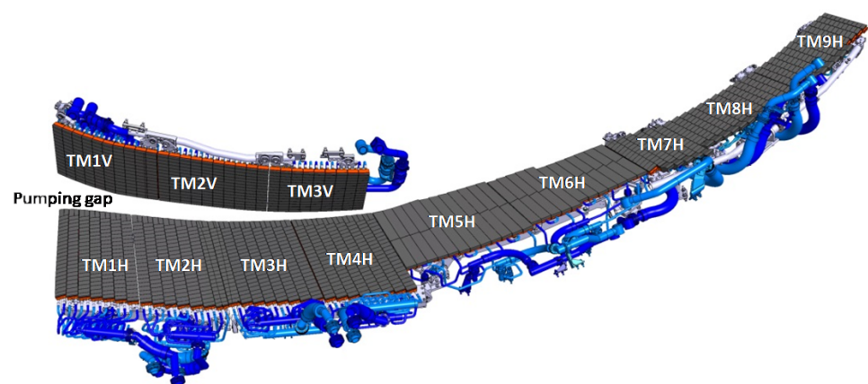
Figure 2. The divertor units are 5 m long and 1 m wide with several target modules: vertical targets (TM1V–TM3V), low- \iota targets (TM1H–TM4H), low-load target modules (TM5H–TM6H) and high- \iota targets (TM7H–TM9H). The divertor water-cooled tiles are made of CFC (Carbon Fibre Composite) except the two low-load central target modules, which are made of fine-grain graphite.
