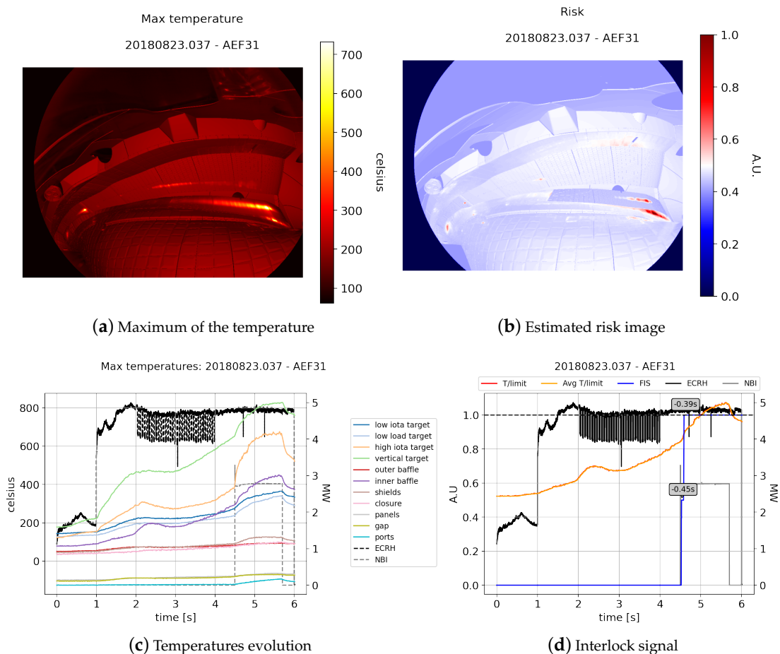
Figure 11. A baffle overload example. (a) Maximum of the temperature over time; (b) Maximum of the estimated risk over time; the strike-lines which are within the temperature limits of the divertor are barely visible; the overload of the baffle stands out. (c) Maximum temperature for each PFCs over time; the inner baffle reaches 400 °C at 5 s. (d) Time evolution of the maximum temperature normalized by the temperature limit over the image, time evolution of the maximum averaged temperature normalized by the temperature limit over the image, and Fast Interlock Signal (0.5 corresponding to a warning and 1.0 to an alarm); We can observe that an alarm is triggered 0.39 s before the maximum temperature reaches the limit (when the baffle temperature reaches 400 °C) well in advance to compensate for the 0.11 s of the system delay.
