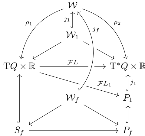
Figure 3.1: Recovering the Lagrangian and Hamiltonian formalisms
