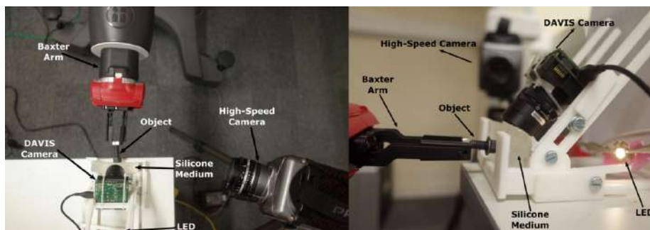
Figure 2.1: Top-down (left) and sideways (right) views of the experiment setup [13].
