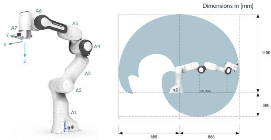
Figure 3.1: Axes of the Panda robotic arm (left) and its work envelope (right) [18].
