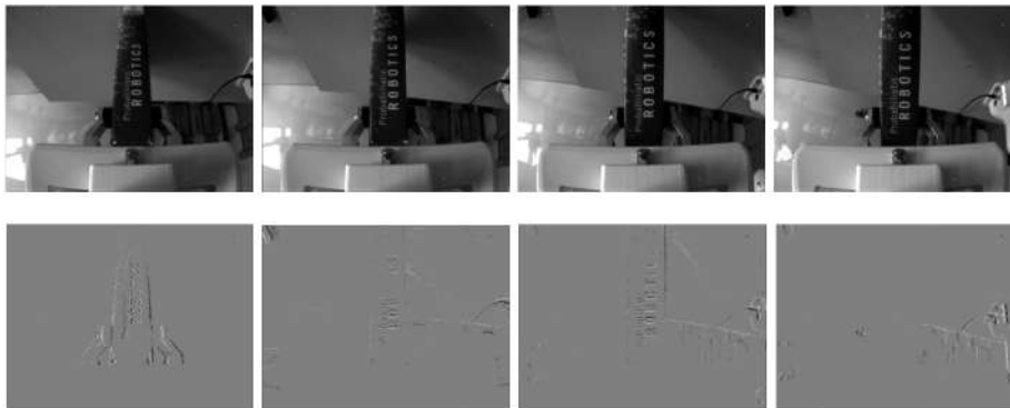
Figure 4.2: Sequence of grayscale frames (first row) and event images (second row) during a slip, while executing a pick-and-place motion with a book.
