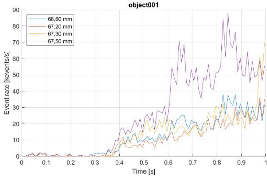
Figure 5.5: Comparison of the event rate evolution in the whole image for 4 samples of object 1 from the dataset in [16].
