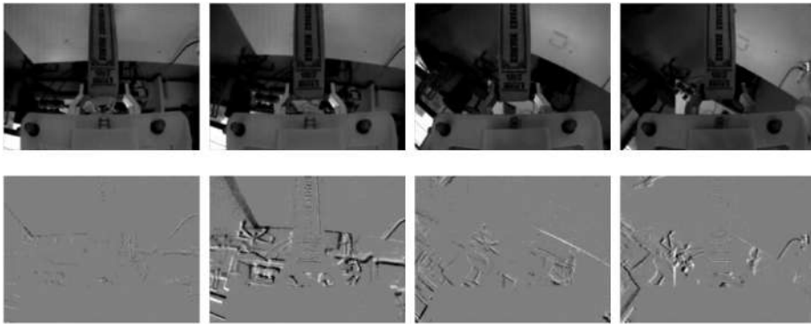
Figure 4.23: Sequence of grayscale frames (first row) and event images (second row) during no slip, while executing a pick-and-place motion with book no. 2.
