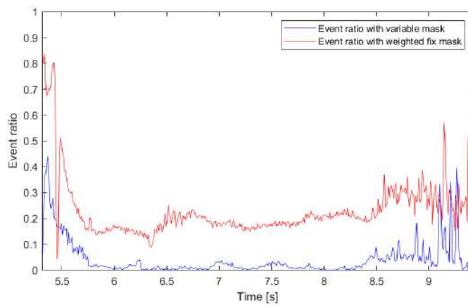
Figure 5.23: Ratio signals of Figure 4.18 using the weighted fix and variable mask.
