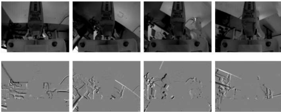
Figure 4.22: Sequence of grayscale frames (first row) and event images (second row) during a significant slip, while executing a pick-and-place motion with book no. 2.
