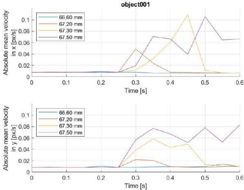
Figure 5.24: Comparison of the absolute mean velocities' evolution in the whole image for 4 samples of object 1 from the dataset in [16].
