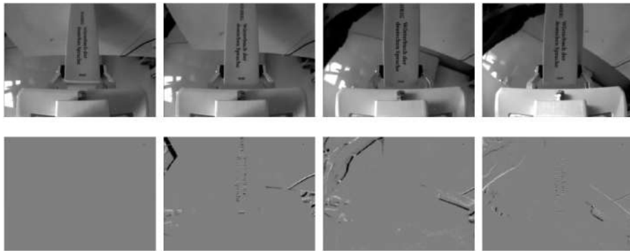
Figure 4.8: Sequence of grayscale frames (first row) and event images (second row) during a significant slip, while executing a pick-and-place motion with book no. 1.
