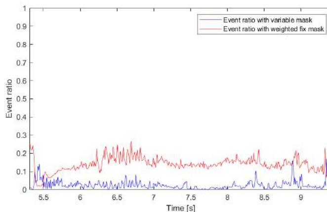
Figure 5.17: Ratio signals of Figure 4.14 using the weighted fix and variable mask.
