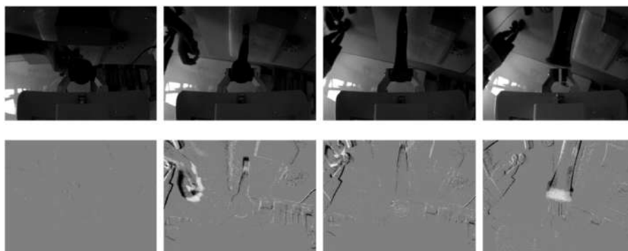
Figure 4.3: Sequence of grayscale frames (first row) and event images (second row) during a grasp failure, while executing a pick-and-place motion with a hammer.
