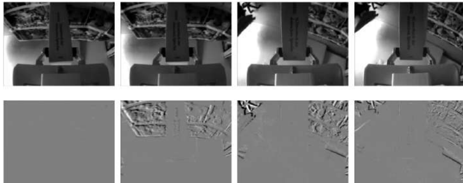
Figure 4.12: Sequence of grayscale frames (first row) and event images (second row) during a significant slip, while executing a pick-and-place motion with book no. 1 and a highly textured table.
