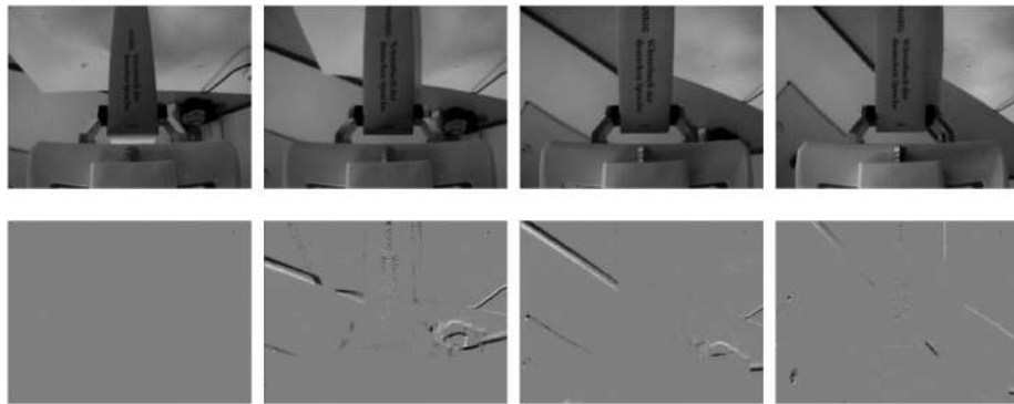
Figure 4.15: Sequence of grayscale frames (first row) and event images (second row) during a significant slip, while executing a pick-and-place motion with book no. 1.
