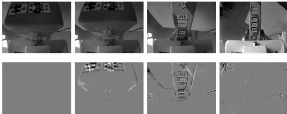
Figure 4.11: Sequence of grayscale frames (first row) and event images (second row) during a significant slip, while executing a pick-and-place motion with a box and reverse grip.
