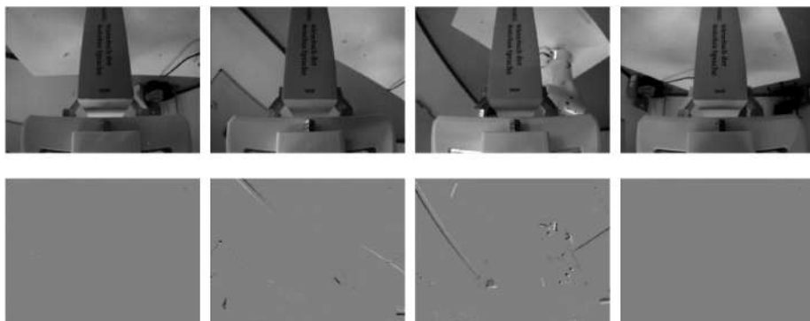
Figure 4.14: Sequence of grayscale frames (first row) and event images (second row) during no slip, while executing a pick-and-place motion with book no. 1.
