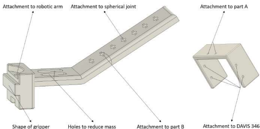
Figure 3.4: Description of the mount: part A (left) and part B (right).
