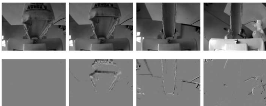
Figure 4.10: Sequence of grayscale frames (first row) and event images (second row) during a significant slip, while executing a pick-and-place motion with book no. 2 and reverse grip.
