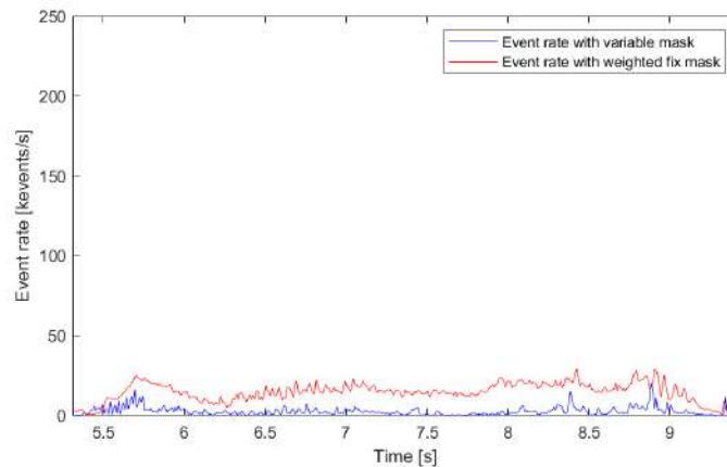
Figure 5.16: Event rate signals of Figure 4.14 using the weighted fix and variable mask.
