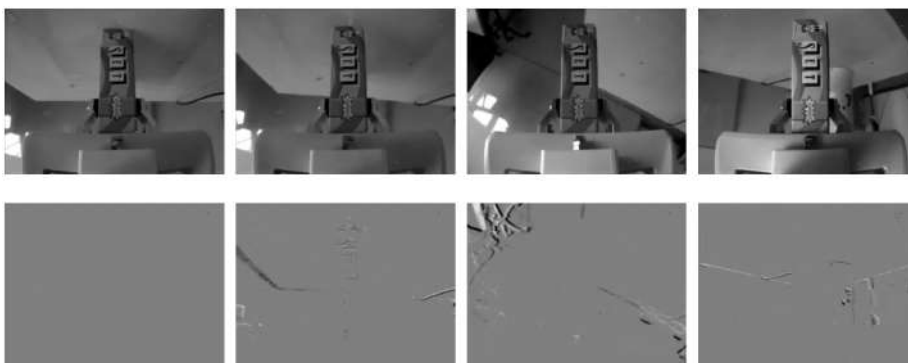
Figure 4.6: Sequence of grayscale frames (first row) and event images (second row) during a minor slip, while executing a pick-and-place motion with a box.
