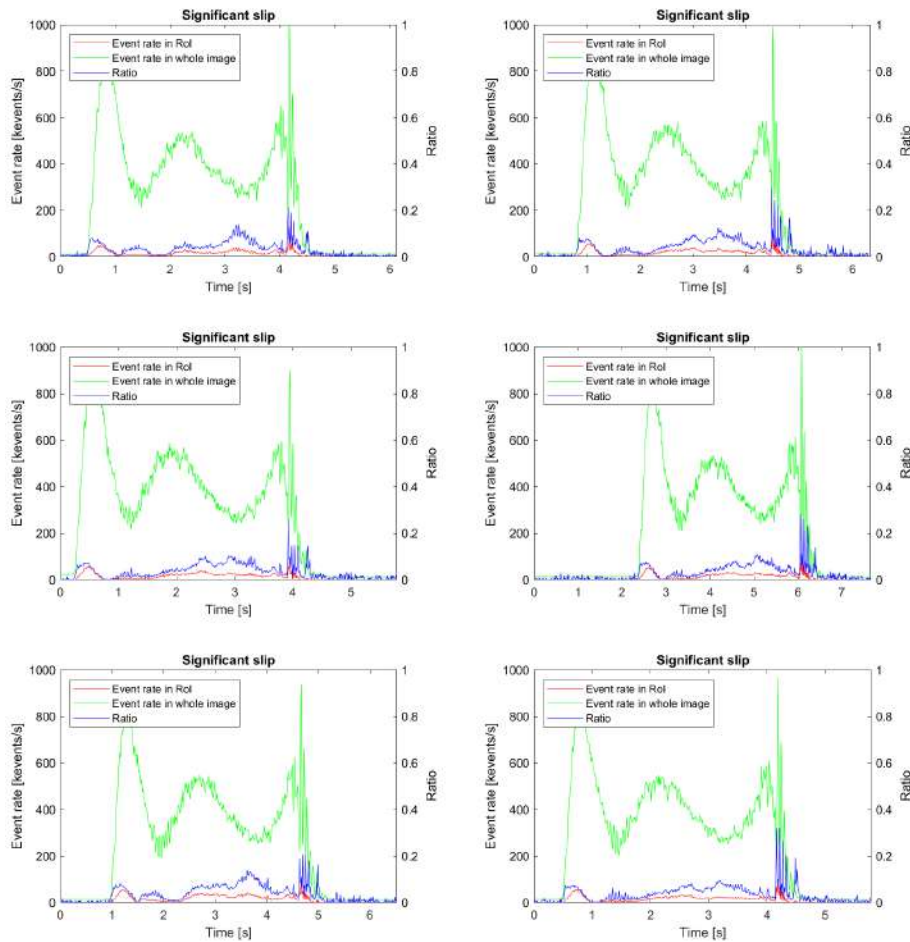
Figure 5.10: Event rate and ratio signals during a pick-and-place motion with book no. 1 and a highly textured table using a fixed RoI.
