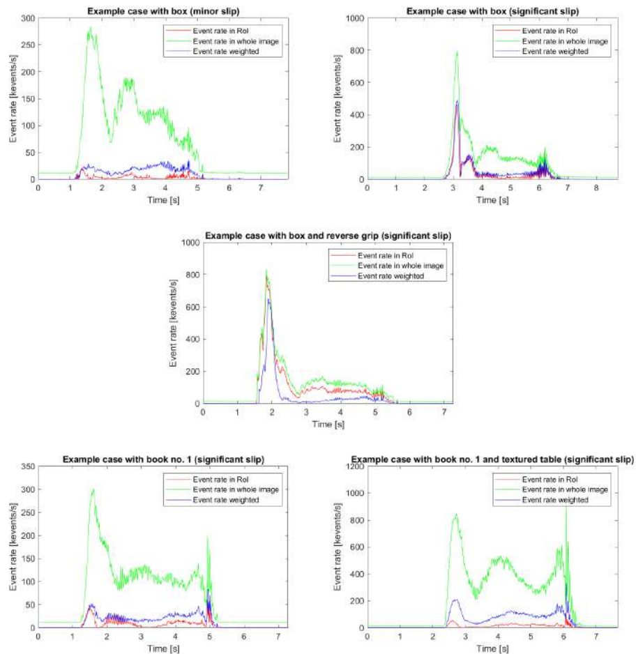
Figure 5.13: Event rate signals during some pick-and-place motions of Set 1 using the fixed RoI and weighted mask.
