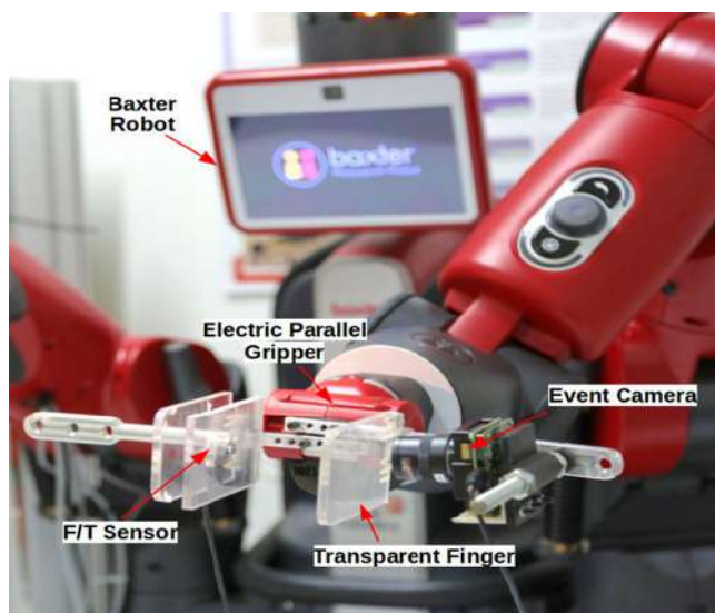
Figure 2.2: Experiment setup: Baxter Gripper with event-based finger prototype [14].
