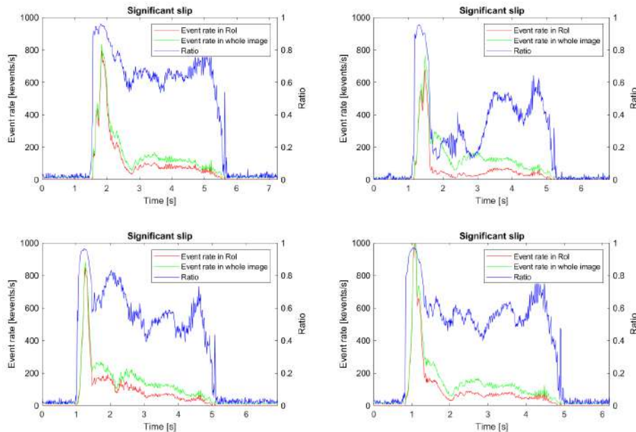
Figure 5.8: Event rate and ratio signals during a pick-and-place motion with a box (reverse grip) using a fixed RoI.
