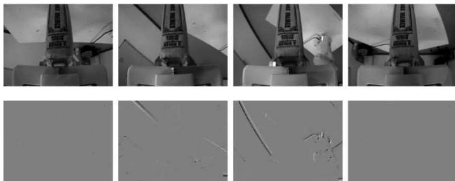
Figure 4.17: Sequence of grayscale frames (first row) and event images (second row) during no slip, while executing a pick-and-place motion with book no. 2.
