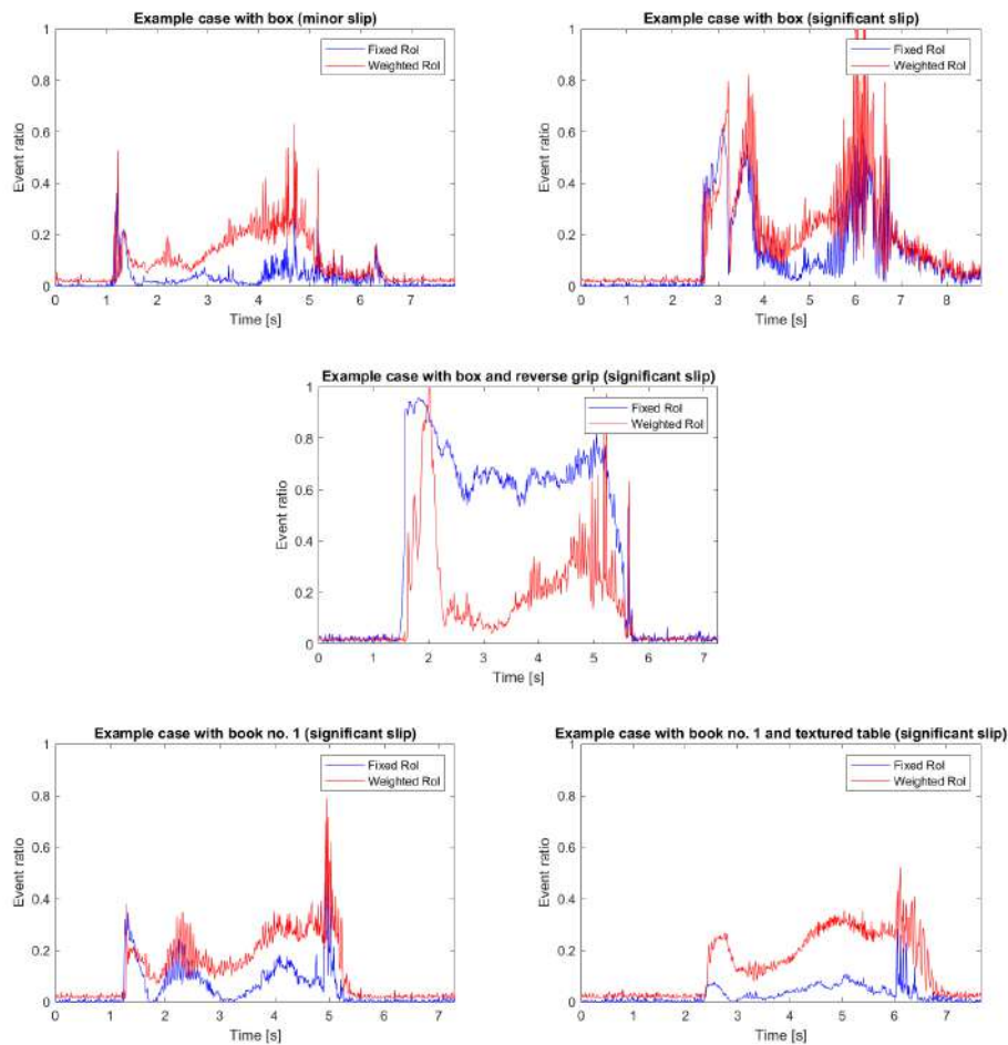
Figure 5.14: Ratio signals during some pick-and-place motions of Set 1 using the fixed RoI and weighted mask.
