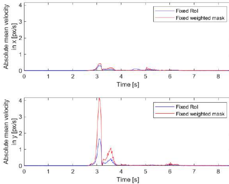
Figure 5.32: Comparison of the absolute mean velocities' evolution in the whole image for the sequence in Figure 4.7.
