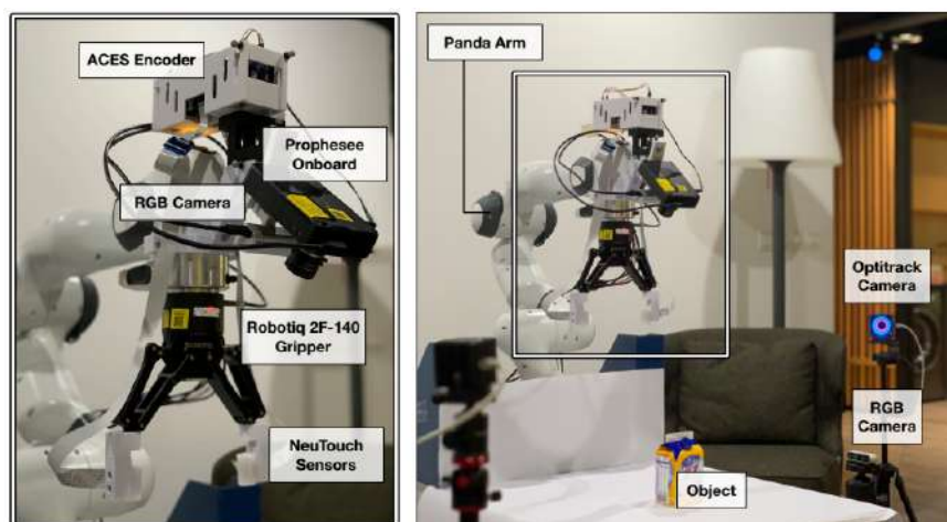
Figure 2.4: Experiment setup: Robot arm, Prophesee event camera, Robotiq gripper, NeuTouch sensors, RGB and OptiTrack cameras [17].
