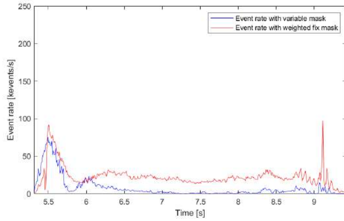
Figure 5.18: Event rate signals of Figure 4.15 using the weighted fix and variable mask.
