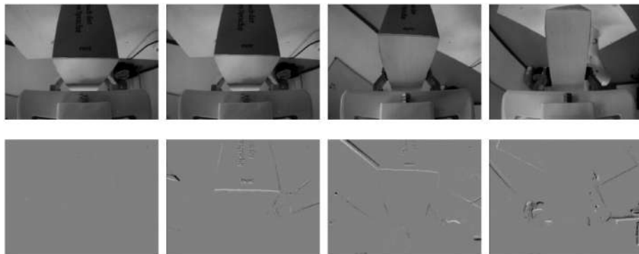
Figure 4.16: Sequence of grayscale frames (first row) and event images (second row) during a significant slip, while executing a pick-and-place motion with book no. 1.
