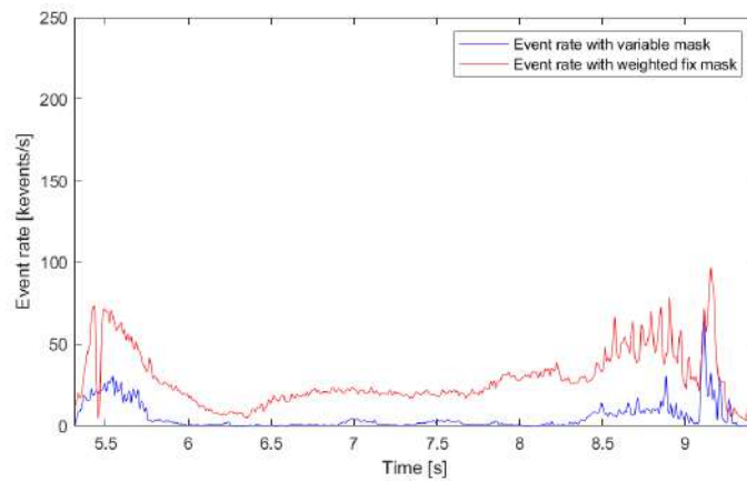
Figure 5.22: Event rate signals of Figure 4.18 using the weighted fix and variable mask.
