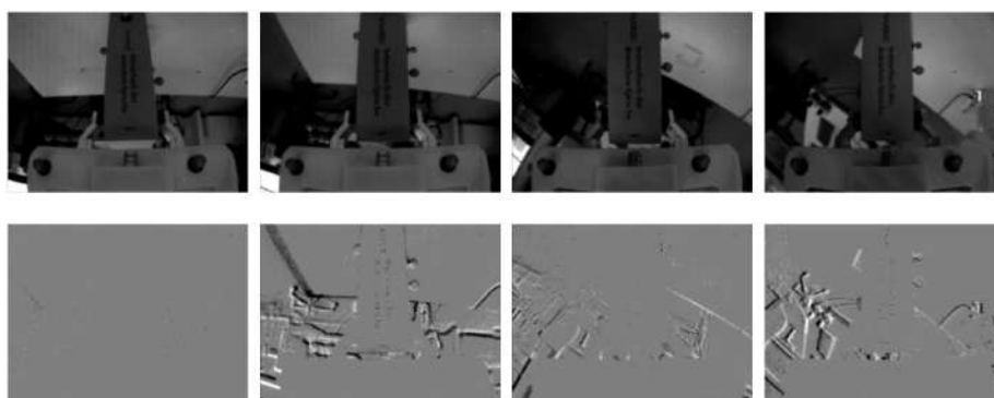
Figure 4.21: Sequence of grayscale frames (first row) and event images (second row) during a significant slip, while executing a pick-and-place motion with book no. 1.
