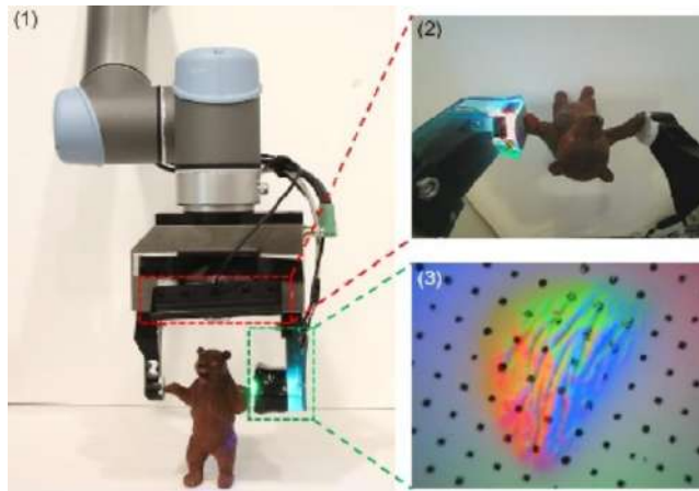
Figure 2.3: (1) Experiment setup: UR5 robot arm with gripper, GelSight sensor and external camera. (2) Image captured by the external camera. (3) Image from GelSight sensor [16].
