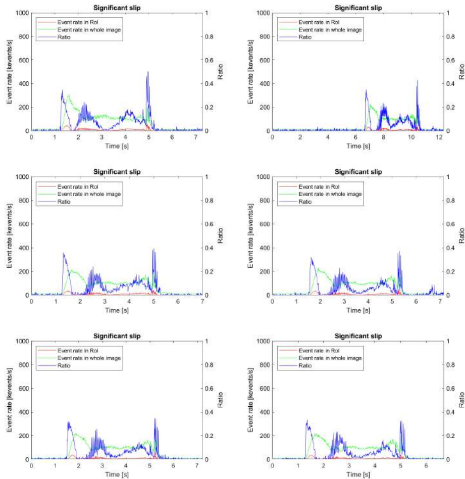
Figure 5.9: Event rate and ratio signals during a pick-and-place motion with book no. 1 using a fixed RoI.
