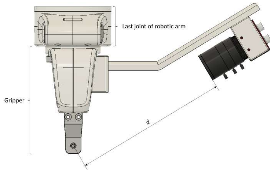
Figure 3.5: Description of the assembly of the mount with the robotic arm, gripper and event-based camera.
