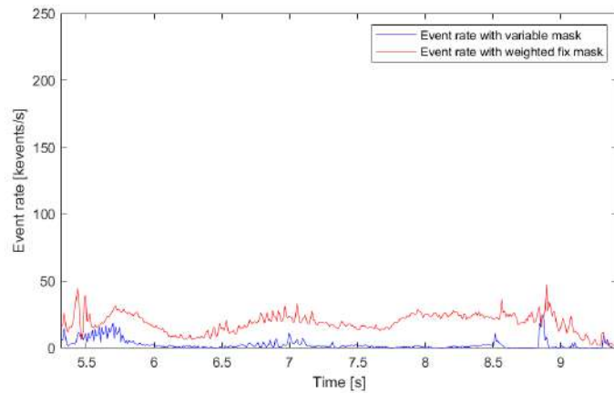
Figure 5.20: Event rate signals of Figure 4.17 using the weighted fix and variable mask.
