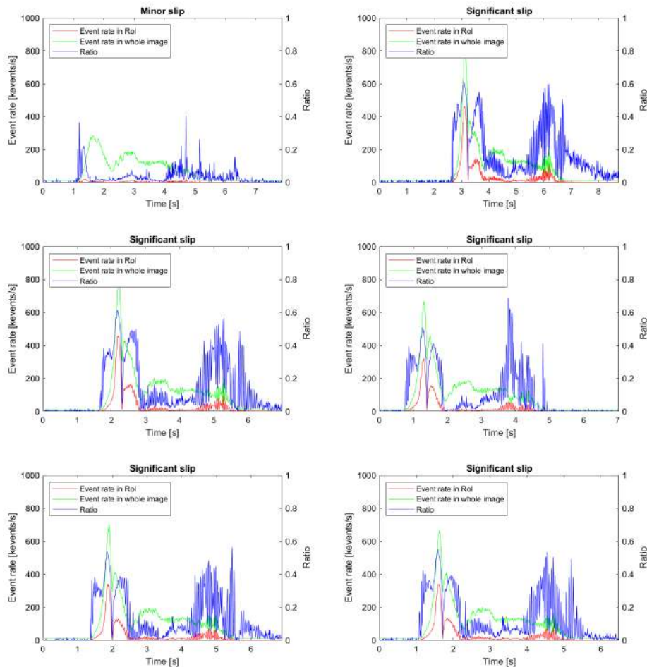
Figure 5.7: Event rate and ratio signals during a pick-and-place motion with a box using a fixed RoI.
