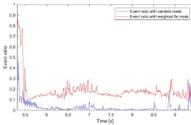
Figure 5.21: Ratio signals of Figure 4.17 using the weighted fix and variable mask.
