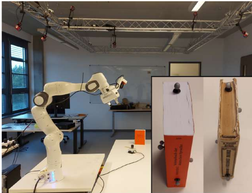
Figure 4.19: Experiment Setup including OptiTrack cameras and objects with markers.
