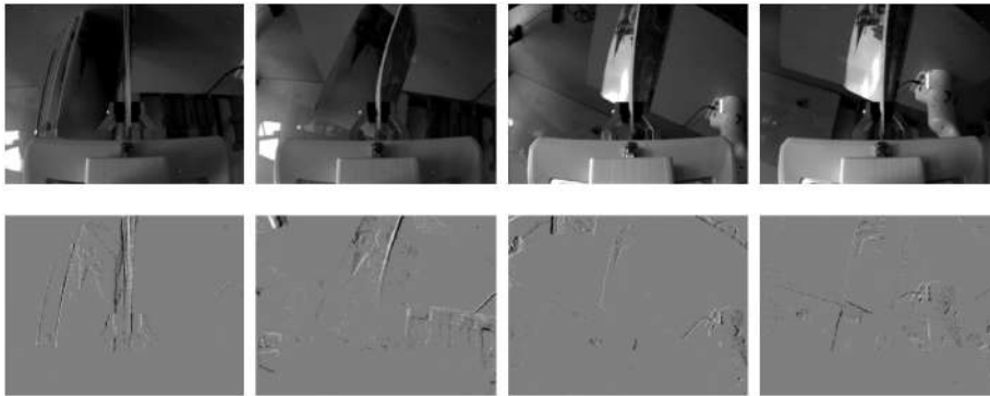
Figure 4.5: Sequence of grayscale frames (first row) and event images (second row) during swinging, while executing a pick-and-place motion with an open book.
