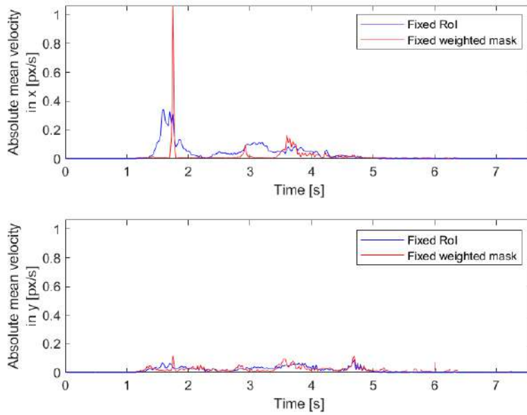
Figure 5.31: Comparison of the absolute mean velocities' evolution in the whole image for the sequence in Figure 4.6.
