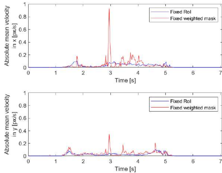
Figure 5.34: Comparison of the absolute mean velocities' evolution in the whole image for the sequence in Figure 4.8.
