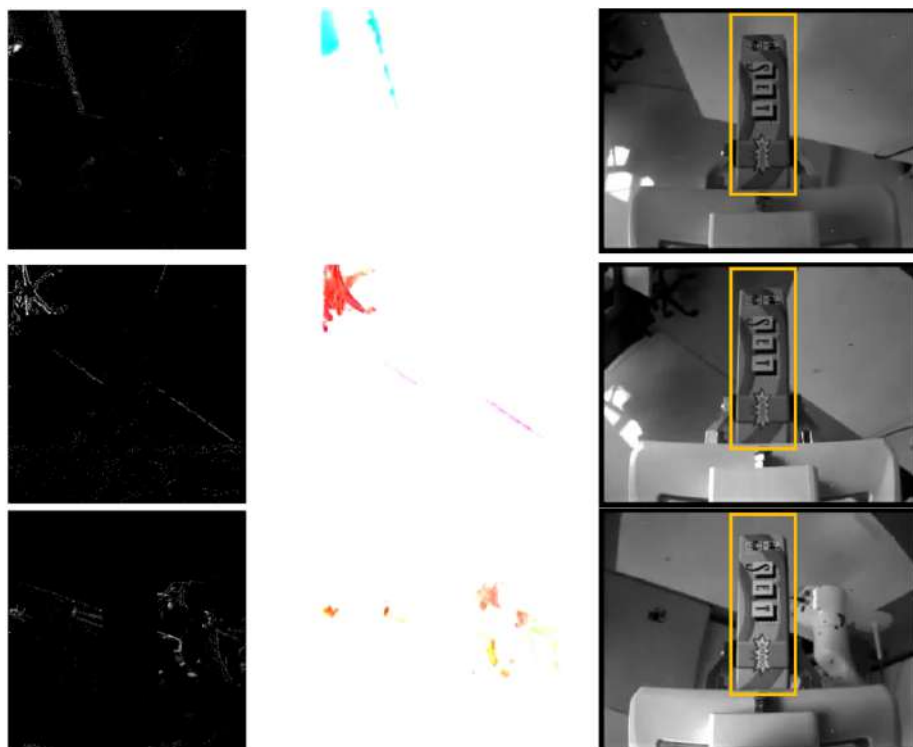
Figure 5.26: Event images (first column), motion flow estimation using optical flow (second column) and grayscale frames (third column) for the sequence in Figure 4.6.
