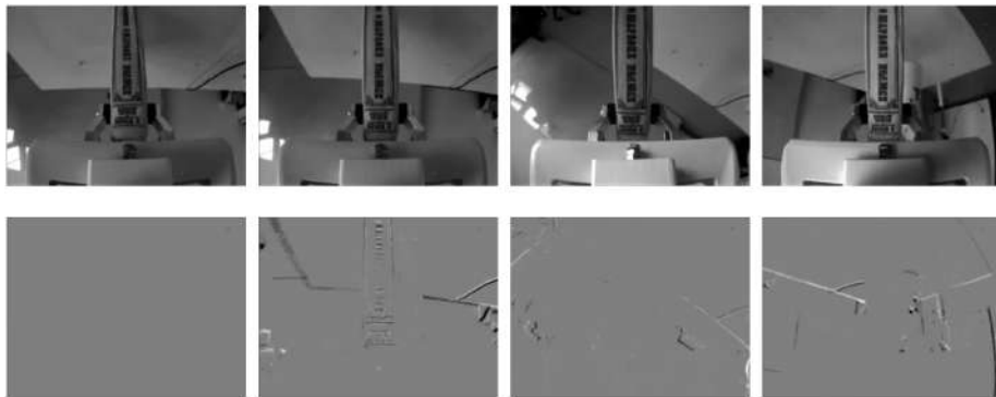
Figure 4.9: Sequence of grayscale frames (first row) and event images (second row) during a significant slip, while executing a pick-and-place motion with book no. 2.
