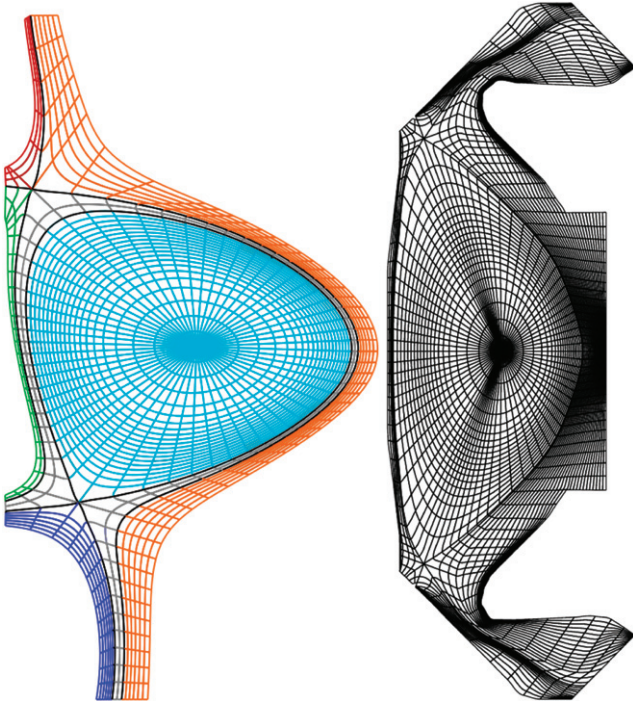
Figure 6. JOREK example grids shown at reduced resolution for clarity. (Left) Flux-surface aligned grid [123] for a TCV equilibrium with two X-points (the lower X-point is active). The part in the closed flux region is shown in light blue, the two separatrices in black, the grid between the separatrices in grey, the lower private flux region in dark blue, the upper private flux region in red, the outer open flux region in orange, and the inner open flux region in green. (Right) Flux surface aligned X-point grid extended to the true first wall (using the methods described in reference [124]) for an MAST Upgrade case with Super-X divertor.
