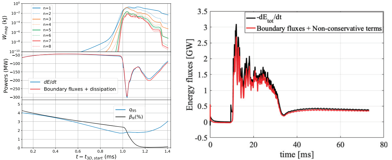
Figure 17. (Left) 3D VDE simulated with JOREK. (Top) Poloidal magnetic energy of the different toroidal harmonics. (Middle) Time derivative of the total plasma energy ( E = W_{mag} + W_{th} + W_{kin} ) and sum of dissipation powers and boundary fluxes (powers representing all energy losses). (Bottom) Evolution of the edge safety factor ( q_{95} ) and of \beta_N during the VDE. The case is explained in detail in [98]. (Right) Time derivative of the total plasma energy and the sum of non-conservative terms and boundary fluxes for a 3D RMP simulation in an ITER 15 MA plasma simulated with JOREK. The simulations includes realistic E \times B and diamagnetic flows and undergoes strong MHD activity between 10 and 35 ms which affects the edge confinement. The case confirms that the error in the energy conservation introduced by gyro-viscous cancelation is small as expected from analytical estimates.
