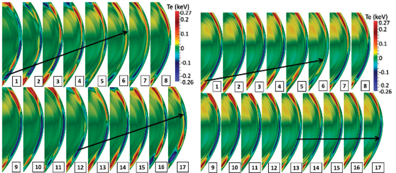
Figure 47. Edge temperature perturbations (non-axisymmetric component) for ASDEX Upgrade simulations of a peeling-ballooning unstable plasma with different RMP amplitudes. The left panel shows different time points during a simulation with moderate RMP amplitude. Edge instabilities form rotating structures of reduced amplitudes compared to the natural ELM crash (mitigation regime). The right panel shows, that a higher RMP amplitude causes a locking of the instabilities. In this case, losses from the plasma are strongly reduced and stationary mode activity is seen (suppression regime). Reprinted from [240], with the permission of AIP Publishing.
