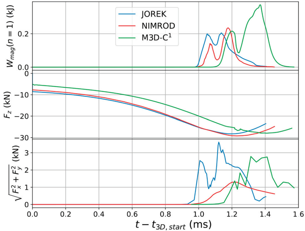
Figure 29. 3D VDE benchmark between JOEKE, NIMROD and M3D-C 1 . The case and comparison is explained in detail in reference [98]. (Top) Magnetic energy of the dominant mode ( n = 1 ). (Middle) Total vertical force. (Bottom) Total horizontal wall force in JOEKE, NIMROD and M3D-C 1 . Re-print from reference [98].
