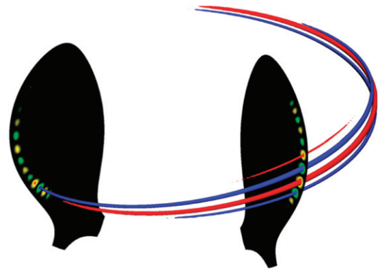
Figure 35. The poloidally and toroidally localized magnetic flux perturbation in an ASDEX Upgrade simulation is shown, which has similarities to so-called solitary MPs observed experimentally [199]. Reprinted from [199], with the permission of AIP Publishing.
