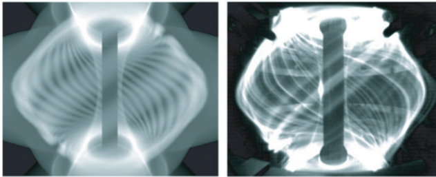
Figure 41. The signature of ELM filaments in visible light is shown for ELMs in MAST. Left: virtual diagnostic data based on a JOREK simulation. Right: visible light picture in the experiment. Reproduced from [226]. © IOP Publishing Ltd. All rights reserved.
