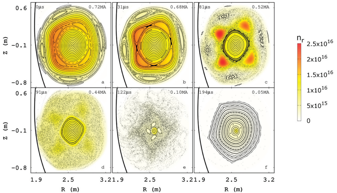
Figure 66. Poincaré plots along with the RE number density (background colour) during the MHD activity leading to the stochastization of the magnetic field and subsequent termination of the RE beam. Remaining RE current is also shown in each panel. Reproduced from [292]. © IOP Publishing Ltd. All rights reserved.
