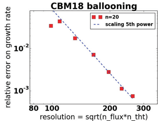
Figure 14. The relative error of the growth rate of a ballooning mode n = 20 is plotted as a function of the spatial resolution \sqrt{n_{\text{flux}} n_{\text{tht}}} , for reduced MHD. The error converges as the 5th power of the spatial resolution, as expected.
