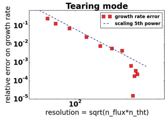
Figure 13. The relative error of the growth rate of a TM is plotted as a function of the spatial resolution \sqrt{n_{\text{flux}} n_{\text{tht}}} , for the full-MHD model. The error converges as the 5th power of the spatial resolution, as expected. Reprinted from [67], with the permission of AIP Publishing.
