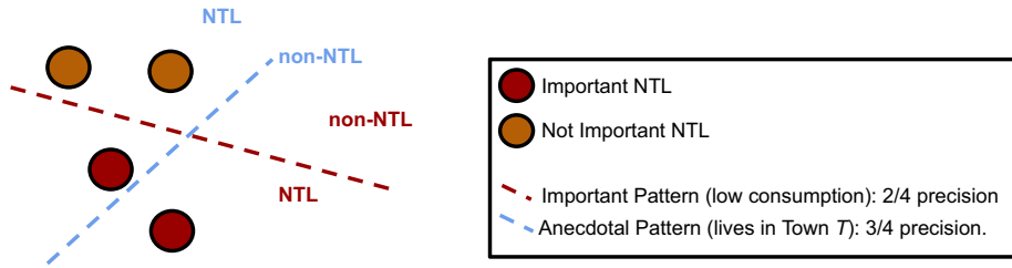
Fig. 2 With the binary classification we are equating the importance of each NTL, learning undesired patterns: if we do not prioritise the darker red instances (NTL cases with a large amount of energy recovered and, therefore, better representatives of the behaviour of an NTL case), we might prioritise undesired patterns like the one represented in a blue pattern. The result is a biased model that cannot robustly detect NTL cases
