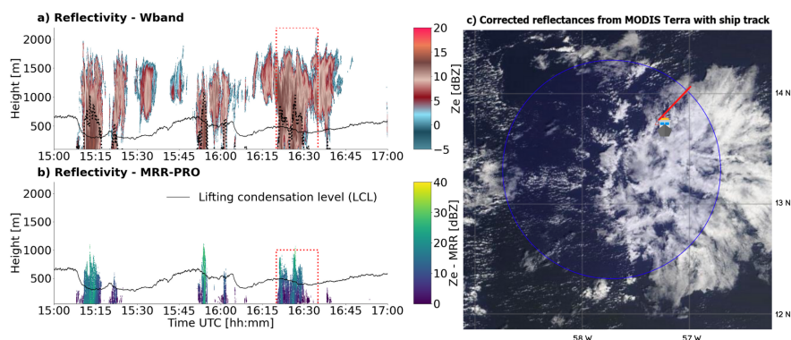
Figure 11. Overview of the selected case study of the 12 February 2020 between 15:00 and 17:00 UTC: a) Radar reflectivity from W-band radar. The black solid line represents the lifting condensation level calculated using the surface variables, while the black dotted line shows the highest detected signal from the MRR-PRO. The red dashed box represents the area shown in Figure 12. b) Attenuated reflectivity from MRR-PRO. c) Ship track on top of the corrected reflectance from MODIS Terra, displaying the flower cloud occurring in the area. The corrected reflectance from MODIS is a product that uses the bands 3 (479 nm, red), 6 (1652 nm, green), and 7 (2155 nm, blue) produced in near real-time (NRT) to provide natural looking images. The blue circle represents the orbit of the HALO aircraft. The image is taken at 16:03 UTC. Source: https://observations.ipsl.fr/aeris/eurec4a/Leaflet/index.html
