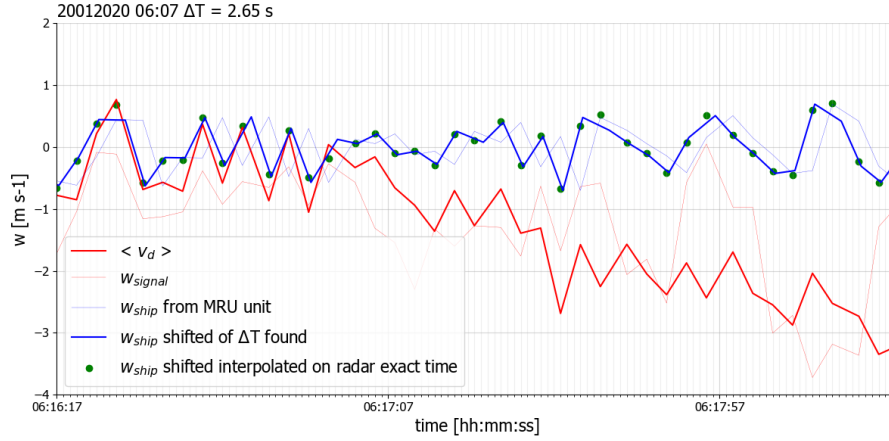
Figure 6. Example of time shift application calculated to obtain the best matched correction for ship motion from the 20 January 2020 over two minutes between 6:16:17 and 6:17:57 UTC. The thin blue line represents the vertical velocity measured by the ship. The thin red line is the mean Doppler velocity recorded by the radar at 1230 m, while the thick red line represents \langle V_d \rangle , the mean Doppler velocity obtained by averaging together all cloudy pixels in each radar profile. The thick blue line represents the ship velocity after applying the time shift of \Delta T = 2.65s , and the green dots represents the values of w_{ship} finally used for correcting for ship motion. They are obtained by cubic interpolation of the shifted ship velocity (thick blue line) on the radar time stamps. In fact, they correspond to the values in the red lines, as expected after interpolation. In the first 7 seconds of the time series, a short train of 3 waves is clearly visible that matches the radar observed mean Doppler velocity values much better after the time shift.
