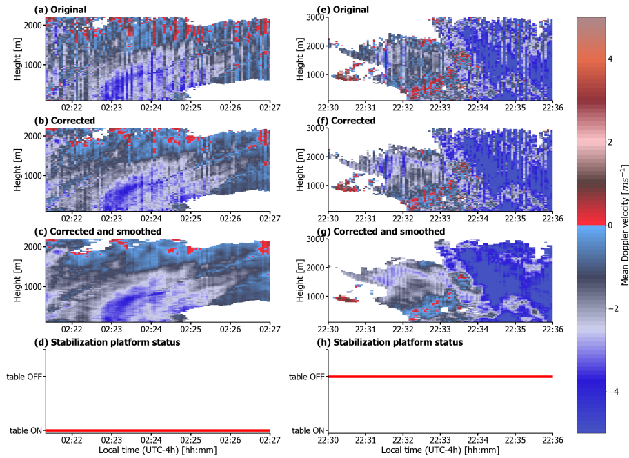
Figure 7. On the left, example of ship motion correction algorithm applied when the stabilization platform was working, on the 20 January 2020 from 2:21 to 2:27 LT (UTC-4h) for the W-band radar data with de-aliasing applied: a) Original mean Doppler velocity field without any correction algorithm applied, b) Mean Doppler velocity after application of the correction from ship motions, c) Mean Doppler velocity after application of correction from ship motions and smoothing (running mean over 9 s), and d) status of the stabilization platform. On the right, another example when the stabilization platform did not work, on the 12 February 2020 between 22:30 and 22:36 LT: e) Original mean Doppler velocity field without any correction algorithm applied, f) Mean Doppler velocity after application of the correction from ship motions, g) Mean Doppler velocity after application of correction from ship motions and smoothing (running mean over 9 s) and h) status of the stabilization platform.
