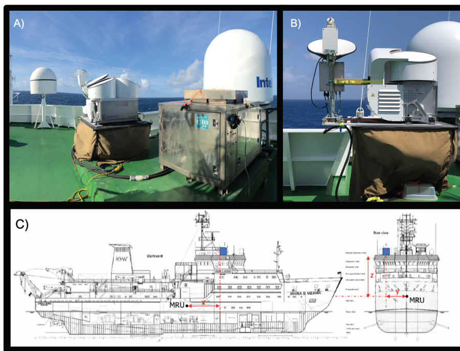
Figure 1. Instrument deployment on the RV MS Merian. A) View of the top deck: the hydraulic unit is visible on the right in the metal box, connected via multiple cables to the stabilization platform. B) The MRR-PRO (left) and the W-band radar (right) fixed using two metal bars on the stabilization platform. C) Position of the instrument deployment with respect to the Motion Reference Unit (MRU) on the MS Merian: side view (left) and front view (right).
