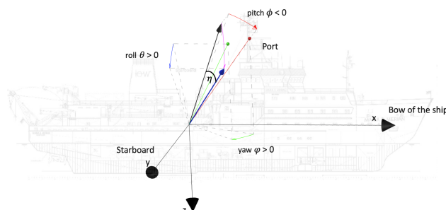
Figure 5. Position of the radar and its tilting due to ship motions expressed in terms of roll, pitch and yaw of the ship. The original position is represented by a black vector (arrow), and the position after the movement is given by a blue arrow. The angle representing the rotation from the initial to the final position is \eta and the roll, pitch and yaw in which it can be decomposed are shown in blue, red and green, respectively. The solid red and green lines ending in filled circles of the same color represent the vector position after undergoing the rotations due first to pitch and then to yaw. The application of the rotation with respect to roll, would then bring the black array on the blue one. The sign with respect to the conventions indicated in the text is reported in the figure.
