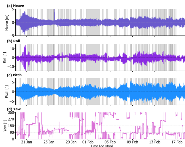
Figure 4. Time series of a) heave, b) roll, c) pitch and d) yaw of the RV MS Merian MRU unit during the EUREC 4 A campaign, from 19 January to 19 February 2020. Grey areas represent the periods of time in which the stabilization platform did not work.
