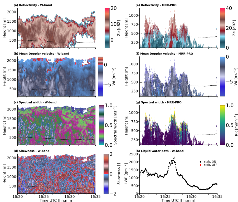
Figure 12. Detail of the case study shown in Figure 11 for W-band variables a) Reflectivity, b) Mean Doppler velocity, c) Spectral width, d) Skewness and for MRR-PRO variables e) Attenuated reflectivity, f) mean Doppler velocity, g) Spectral width. LWP and stabilization platform status are displayed in h).
