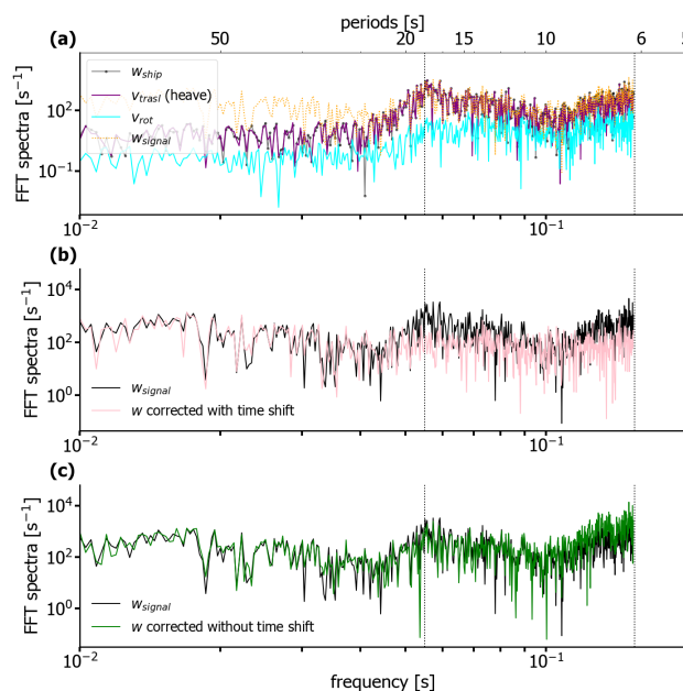
Figure 8. a) Fast-Fourier Transform (FFT) of the ship vertical velocity and of its translational (purple) and rotational (cyan) components for one hour of data collected at a cloudy range gate located at 1605 m from the radar. The ship velocity highlights two main wave periods around 6 and 17 seconds, indicated by dashed vertical lines. In the total ship velocity (black dotted line), the contribution of the rotational component is minor compared to the contribution of the translational component (heave). b) Comparison of the FFT of the radar uncorrected mean Doppler velocity (black) and of the FFTs of the corrected mean Doppler velocity with time shift applied. The two main wave peaks disappeared in the corrected signal (pink line). c) Same as middle panel, but with the corrected mean Doppler velocity calculated without applying the time shift. In this case, the wave frequencies are not removed from the corrected signal (green line).
