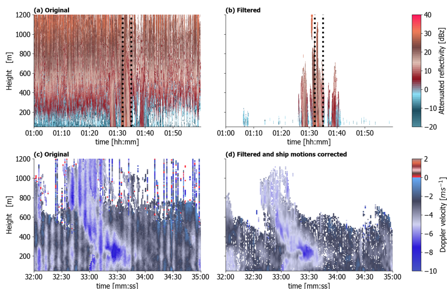
Figure 9. a) MRR-PRO attenuated reflectivity on the 13 February 2020 at 1:00 UTC after manufacturer processing, without any additional interference filtering or ship motion correction. b) Same as a), but with the noise removal mask applied. c) MRR-PRO mean Doppler velocity without any correction over a 2 min time interval selected from the time interval shown in a) between 1:32 and 1:35, and b) and highlighted with dashed black lines. Vertical stripes structures are visible due to ship motions. d) Same as c) but with interference removed and time shift and ship motion corrections applied to the data. The striped structure present in c) almost entirely disappeared and made a hook rain structure visible, possibly caused by downdraft wind mixing.
