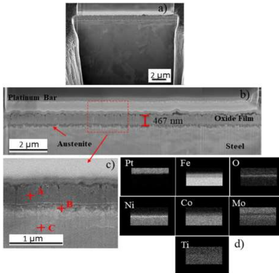
Figure 18 - Scanning electron microscope (SEM) micrographs of the oxide layer formed in maraging 300 alloy, (a) focused ion beam (FIB)-cross section micrograph of the oxide layer, (b) thickness of the oxide layer, (c) magnification of the oxide layer showing the three different points where the chemical composition were determined, and (d) energy-dispersive X-ray spectroscopy (EDS) maps analysis for different metallic elements present in the oxide later (Fe, O, Ni, Co, Mo and Ti) in the region described in Figure 18c.
