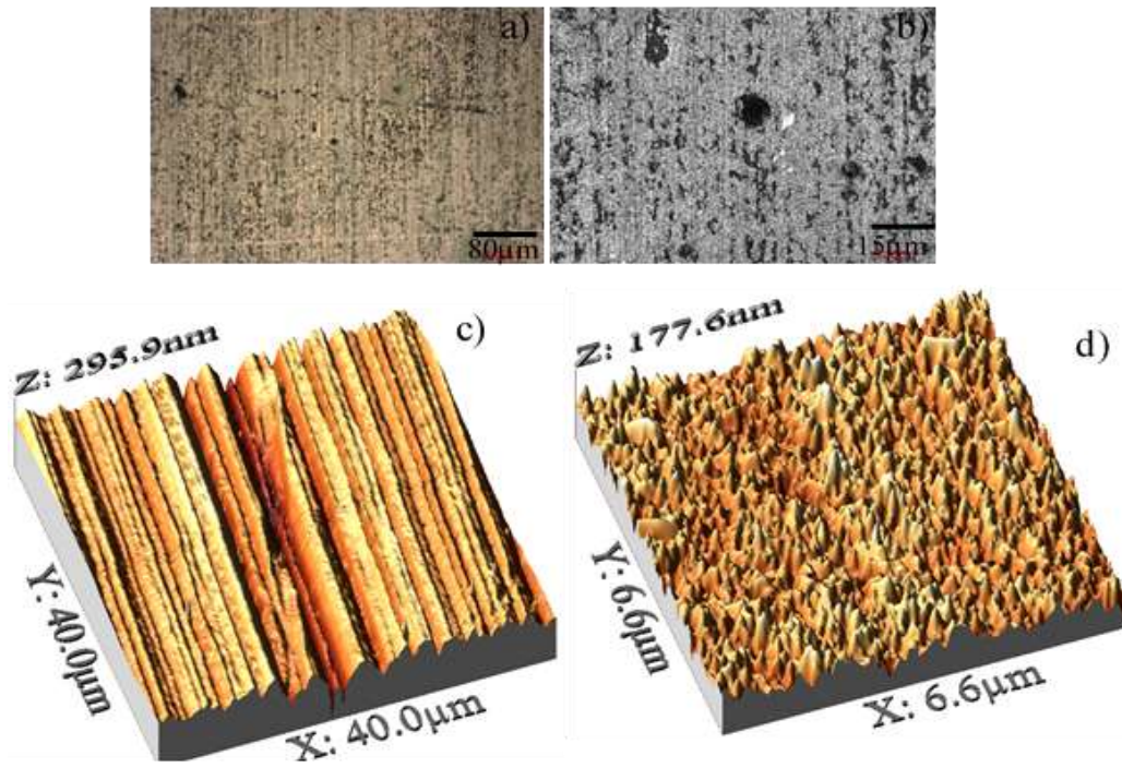
Figure 14 - (a,b) laser scanning confocal microscopy (LSCM) surface micrographs observation, and topographic atomic force microscopy (AFM) image (3D view) of the (c) initial surface and (d) the oxide layer growth on maraging 300 alloy.
