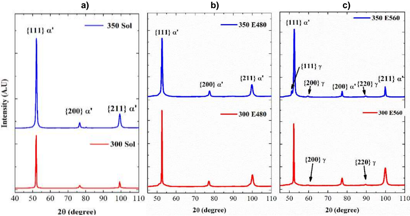
Figure 6 - X-ray diffraction pattern of the grade 300 and 350 maraging steel samples solution treated at 840 °C (5a), aged at 480 °C for 3 h (5b), and aged at 560 °C for 1 h (5c).
