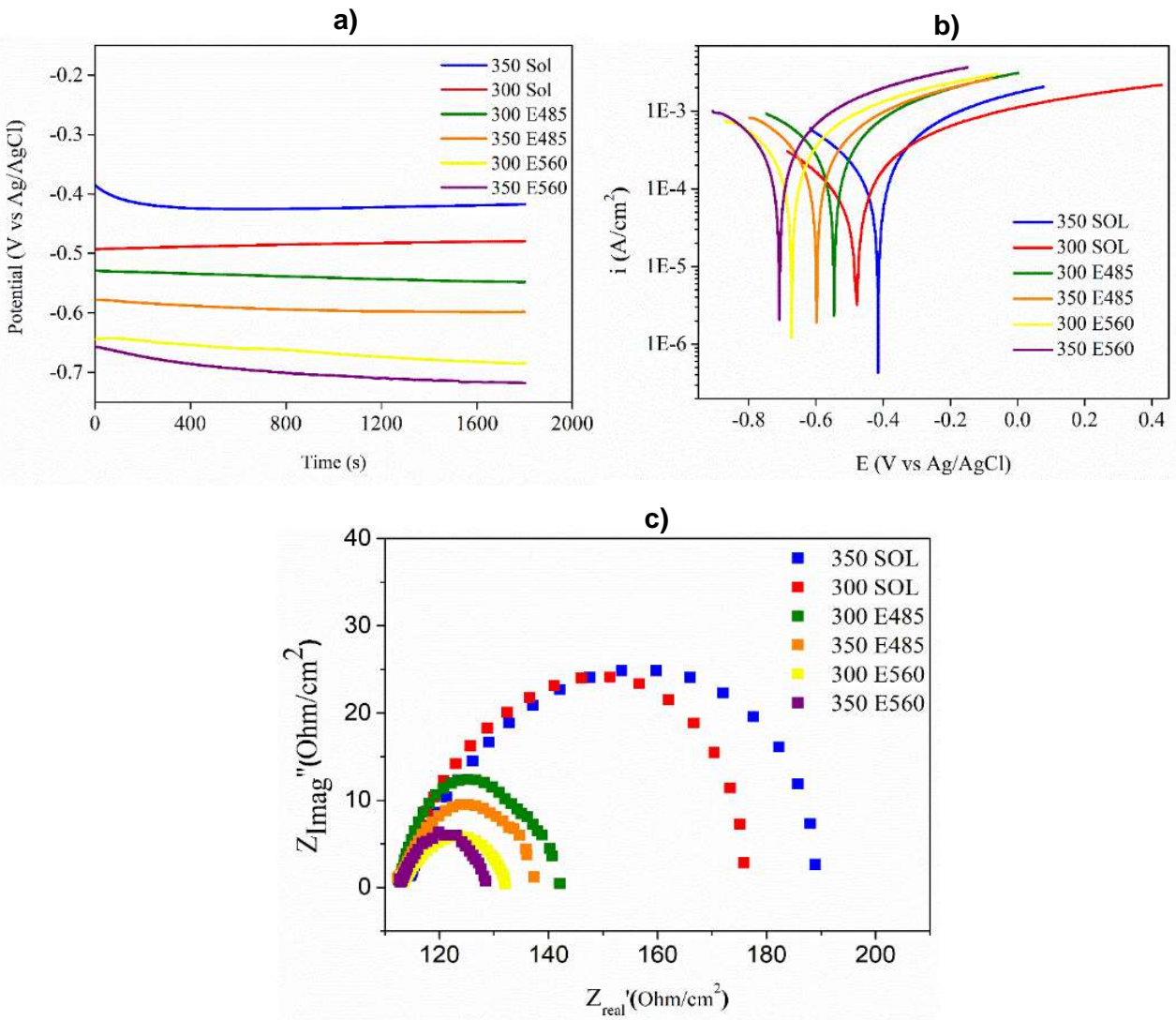
Figure 8 - OCP curves (8a), Linear polarization curves (8b) and EIS (Nyquist) curves (8c) of the grade 300 and 350 maraging steels in 0.01M HF aqueous solution.
