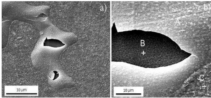
Figure 40 - Scanning electron microscopy (SEM) micrographs of the oxide formed on Mar350 maraging steel: (a) different heterogeneities found on the surface of the oxide and (b) magnification of a broken area of the oxide (A: protuberance on the oxide, B: internal part of the oxide, and C: more homogeneous part of the oxide).
