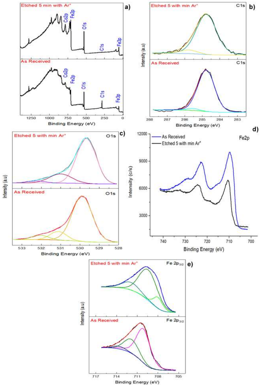
Figure 57 - XPS spectra of the oxide formed on maraging steel 350 before (As received) and after etching 5 min with Ar + plasma (Etched 5 min Ar + ). a) survey spectrum, b) C 1s, c) O 1s, d) Fe 2p and e) Fe 2p 3/2 deconvoluted.
