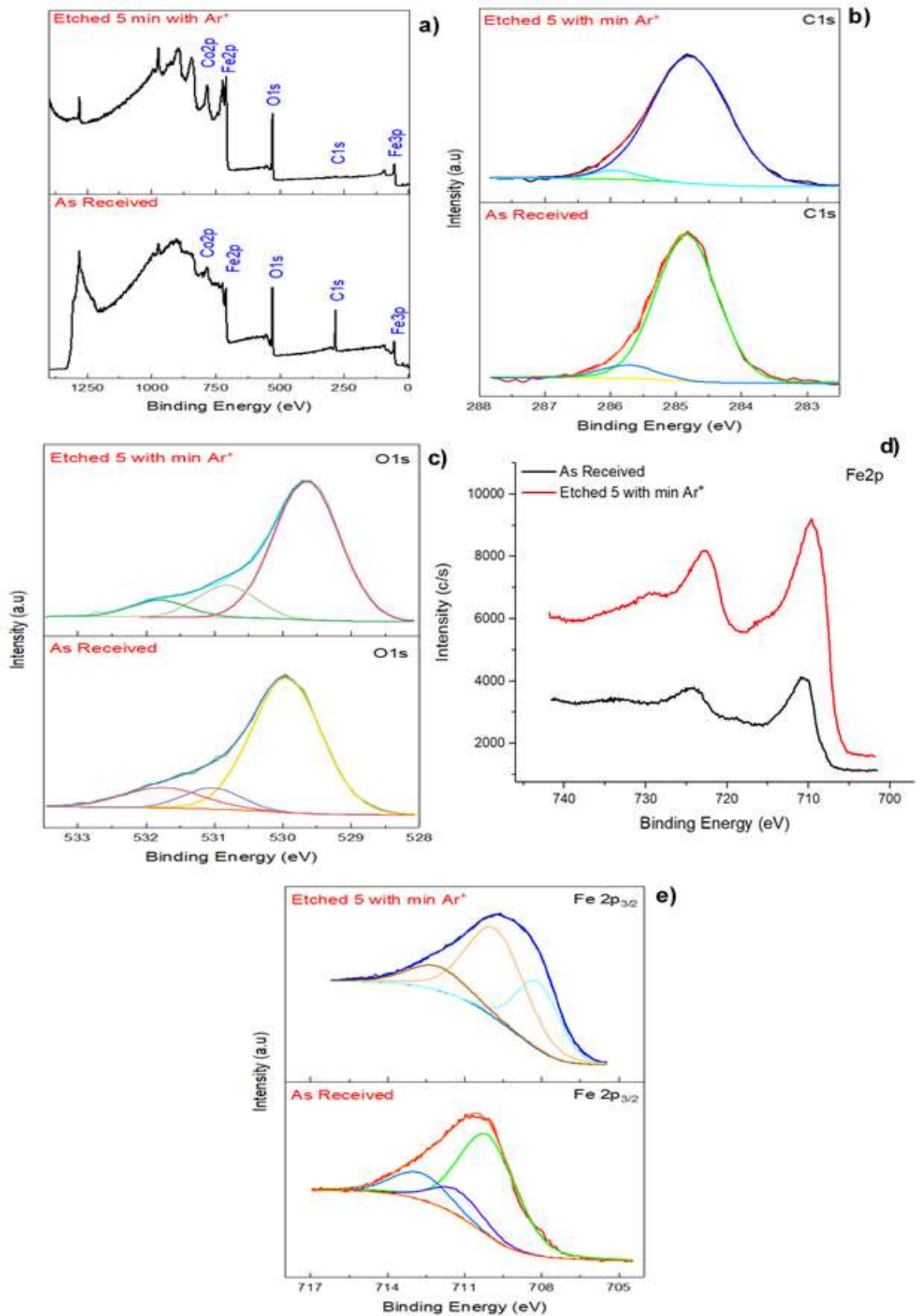
Figure 56 - XPS spectra of the oxide formed on maraging steel 300 before (As received) and after etching 5 min with \text{Ar}^+ plasma (Etched 5 min \text{Ar}^+ ). a) survey spectrum, b) C 1s, c) O 1s, d) Fe 2p and e) Fe 2p_{3/2} deconvoluted.
