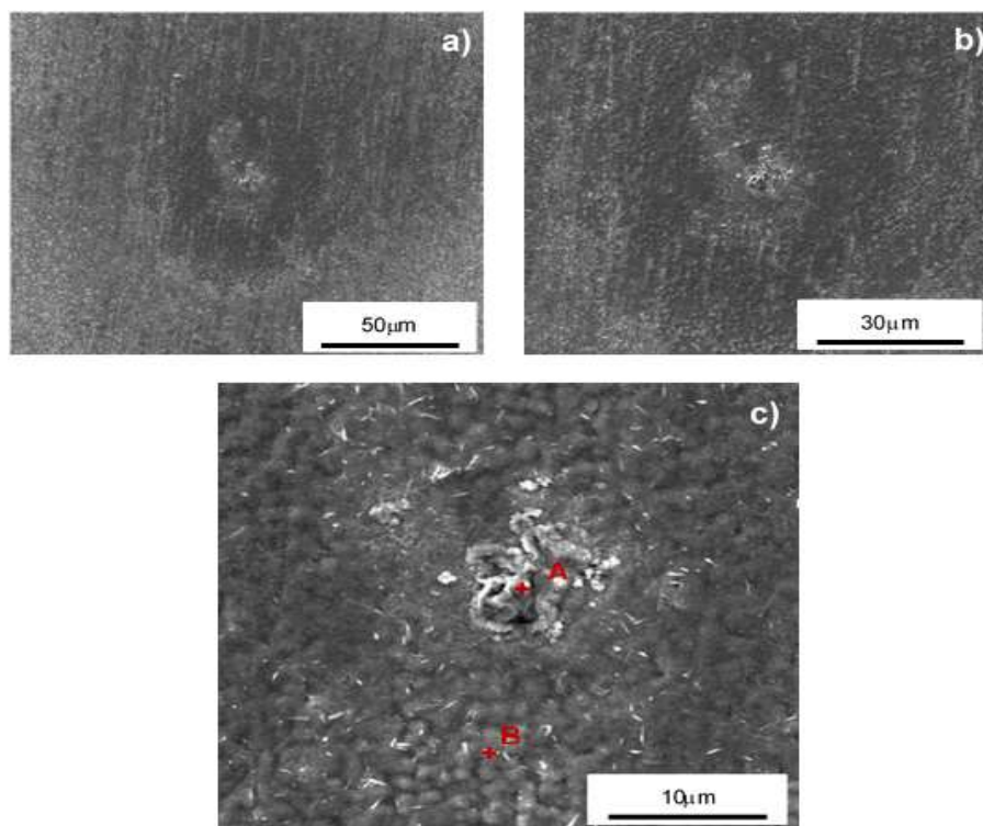
Figure 29 - Scanning electron microscopy (SEM) micrographs of the oxide layer growth under O 2 /steam/N 2 atmosphere on maraging 350 alloy.
