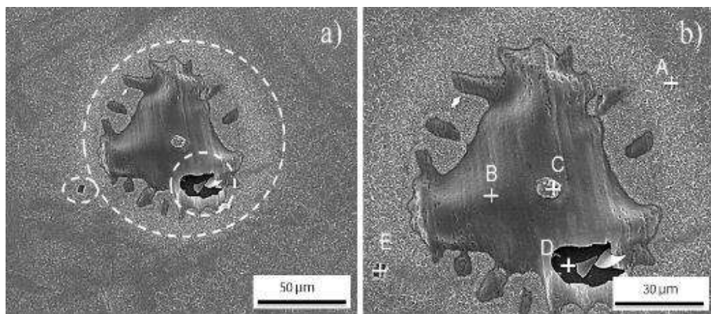
Figure 38 - Scanning electron microscopy (SEM) micrographs of the oxide formed on Mar300 maraging steel, (a) different heterogeneities found on the surface of the oxide and (b) magnification of the defects found on the oxide.
