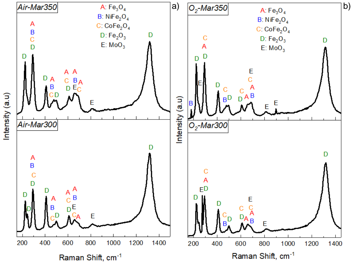
Figure 31 - Raman spectra of the oxide layer growth under different atmospheres on maraging 300 and 350 alloy.
