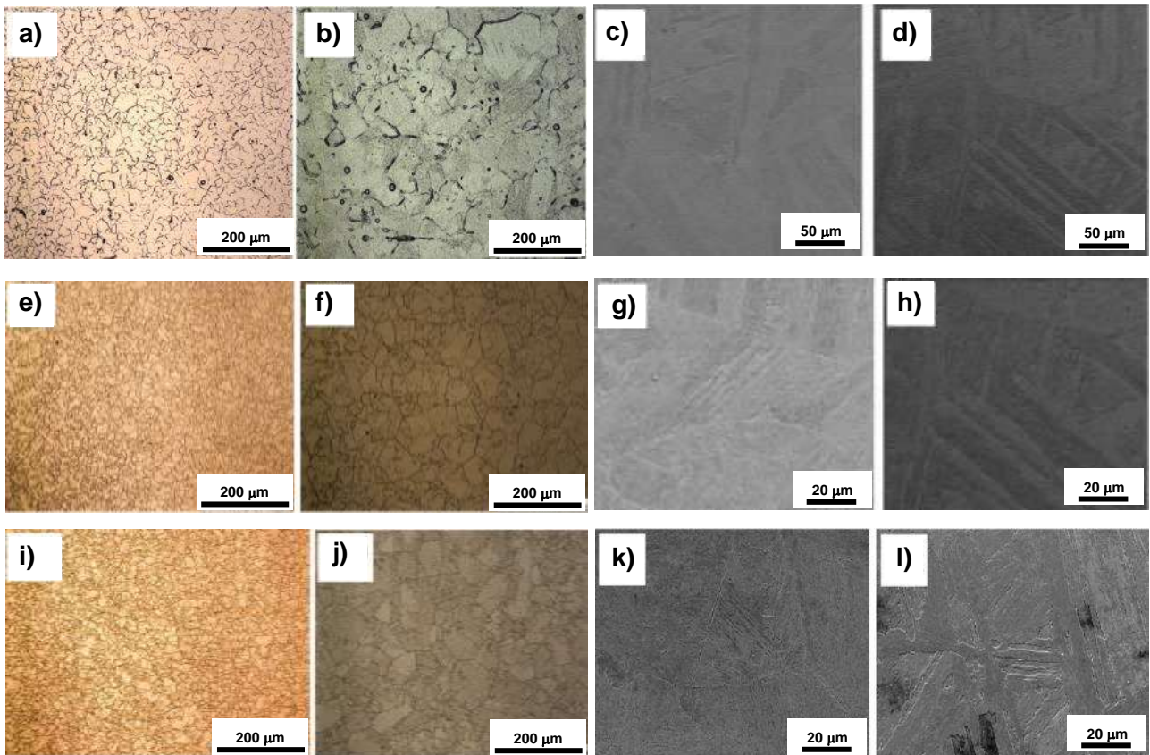
Figure 5 - Optical microscopy images and SEM of the microstructure of the solution annealed at 840 °C, aged at 480 °C and aged at 560 °C conditions.
