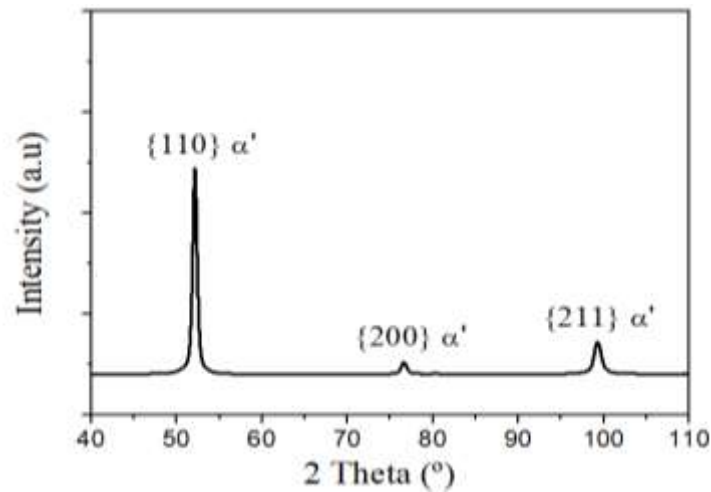
Figure 12 - X-ray diffraction (XRD) spectrum of the maraging 300 alloy after solution annealing treatment at 840 °C showing \alpha' -peaks.
