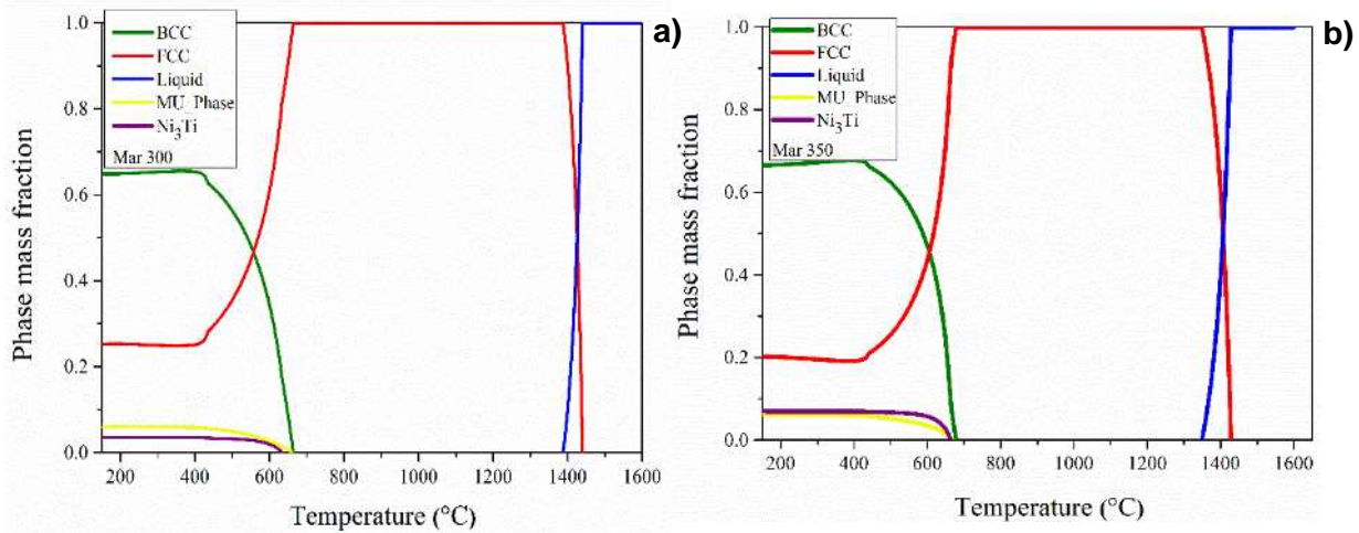
Figure 4 - Mass fraction diagram of grade 300 and 350 maraging steel.
