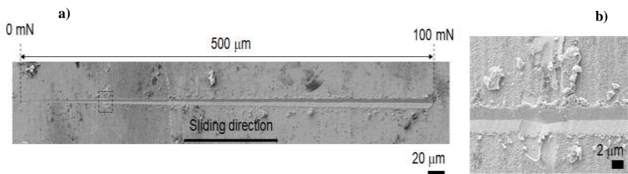
Figure 20 – (a) Field emission scanning electron microscopy (FE-SEM) micrograph for the nanoscratch track and (b) magnification of the top-view (FE-SEM) image of nanoscratch tracks where the first adhesive damage appears for the reference sample.
