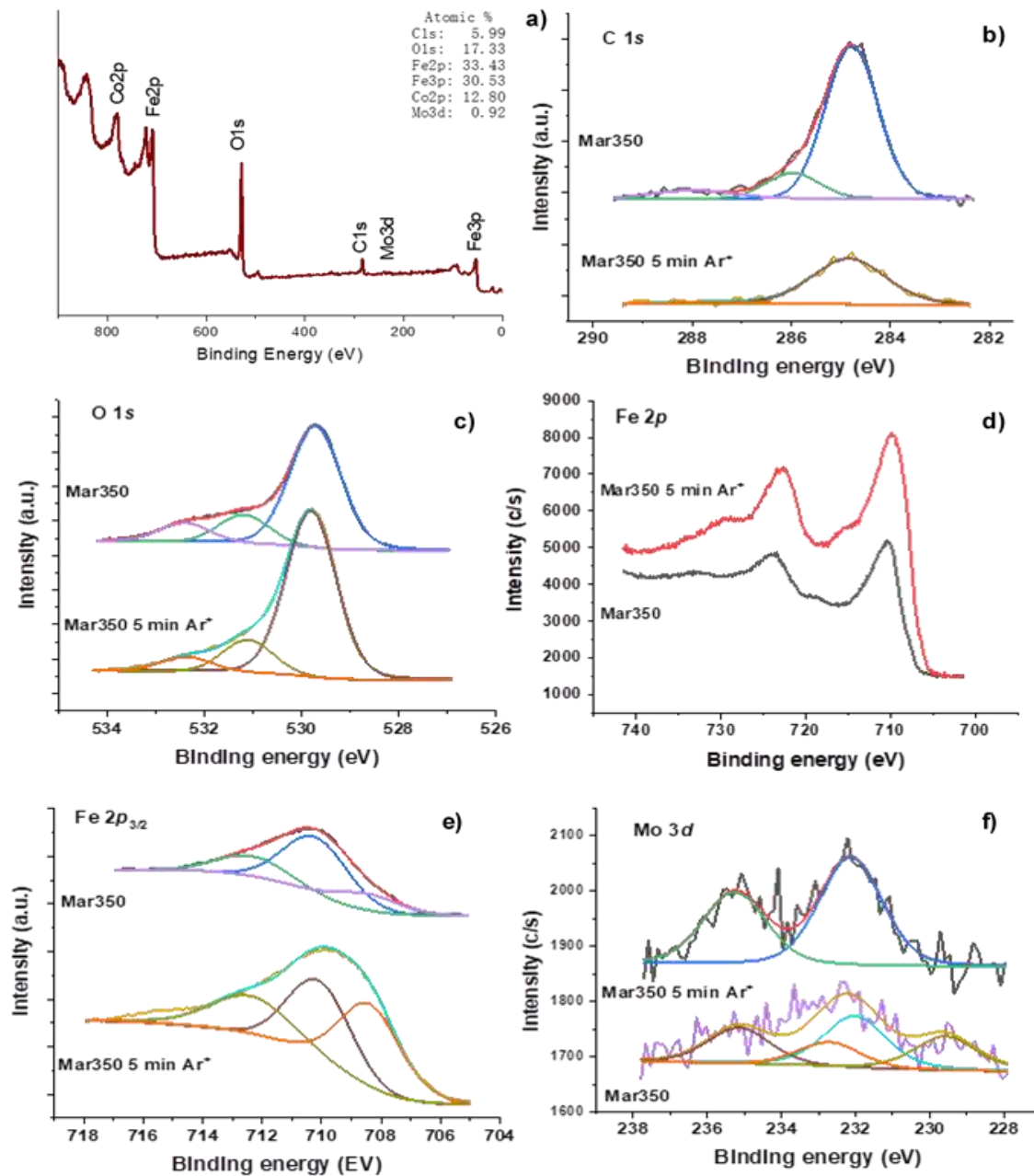
Figure 47 - X-ray photoelectron spectroscopy (XPS) spectra of samples with the oxide produced on grade 350 maraging steel before (Mar350) and after etching for 5 min with Ar + plasma (Mar350 5 min Ar + ). (a) Survey spectrum of sample, (b) C 1s, (c) O 1s, (d) Fe 2p, (e) Fe 2p 3/2 deconvoluted, and (f) Mo 3d.
