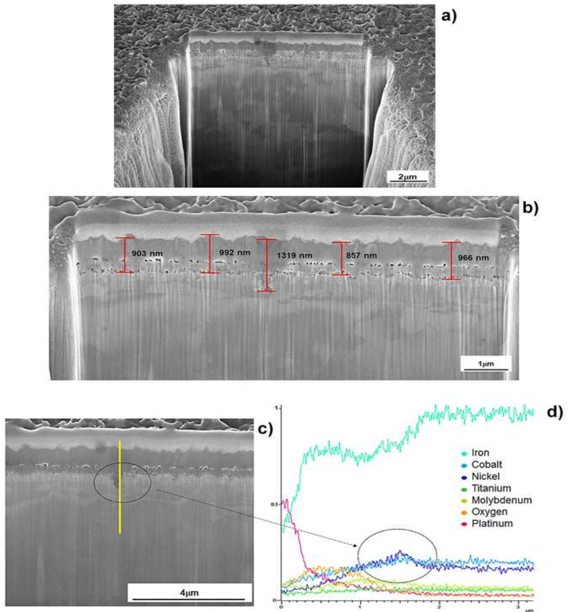
Figure 53 - Scanning electron microscope (SEM) micrographs of the oxide layer formed on maraging 300 steel, (a) focused ion beam (FIB) cross section micrograph of the oxide layer, (b) thickness of the oxide layer, (c) magnification of the oxide layer showing a yellow line where the chemical composition was determined, and d) energy-dispersive X-ray spectroscopy (EDS) chemical elements profiles conducted on the through the yellow line of the Figure 53c.
