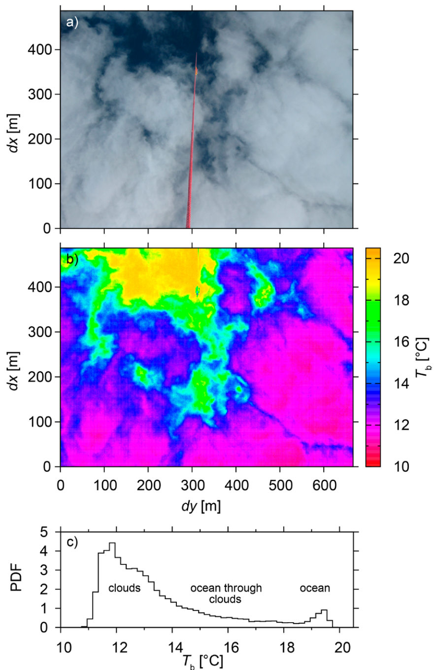
Fig. 13. (a) Image of the cloud in the visible wavelength range taken from above the cloud looking in nadir direction. (b) Infrared image from the GOBI camera for the same image section. (c) Corresponding PDF of the brightness temperature, showing two maxima for cloud and ocean temperatures and a broad transition zone between both maxima where the ocean is visible through the clouds.
