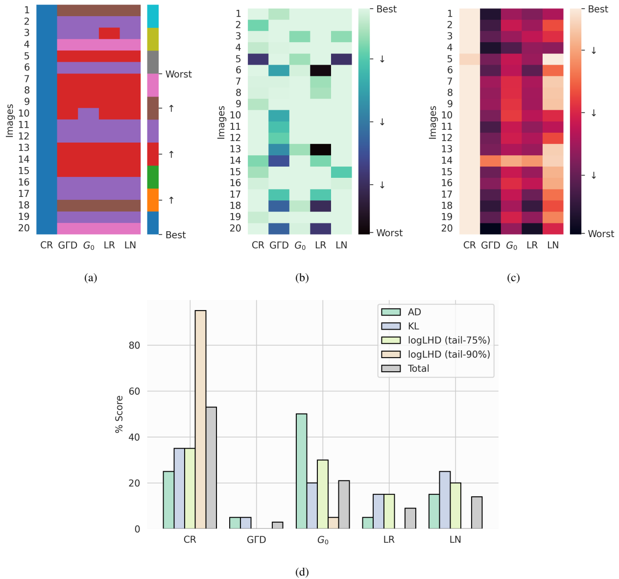
Fig. 4. Modeling performance analysis. Heatmap representations of (a) RSE, (b) KS p -values, and (c) AICc. (d) Percentages of being the best model among 20 images in terms of the measures of KL, AD, LogLHD and Total. To calculate the Total % Score, all statistical models are assessed in terms of RSE, AICc, KL, AD, and p -value measures. For each measure, percentages of being the best model are calculated and combined to obtain Total % Score (E.g. 50% means being the best models in terms of the half of the error measures). CR: Cauchy-Rician, LR: Laplace-Rician, LN: Lognormal.
