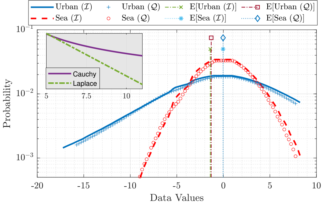
Fig. 2. Comparison for \mathcal{I} and \mathcal{Q} components of different SAR scenes. Mini-figure with darker background: Laplace pdf vs. Cauchy pdf.
