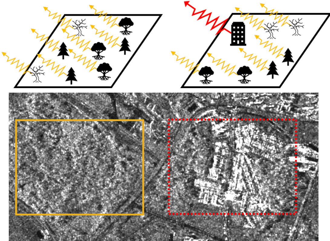
Fig. 1. Surface scattering examples. (left): distributed scattering. (right): a number of strong scatterers.
