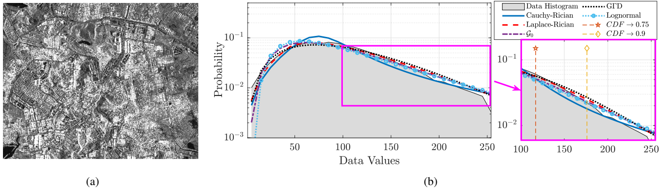
Fig. 5. Visual evaluation of SAR amplitude models. (a) Urban SAR Scene. (b)-(left) Log-pdf of SAR image in (a) and model fits. (b)-(right) The zoomed-in axis for the tail of the histogram with model fits.
