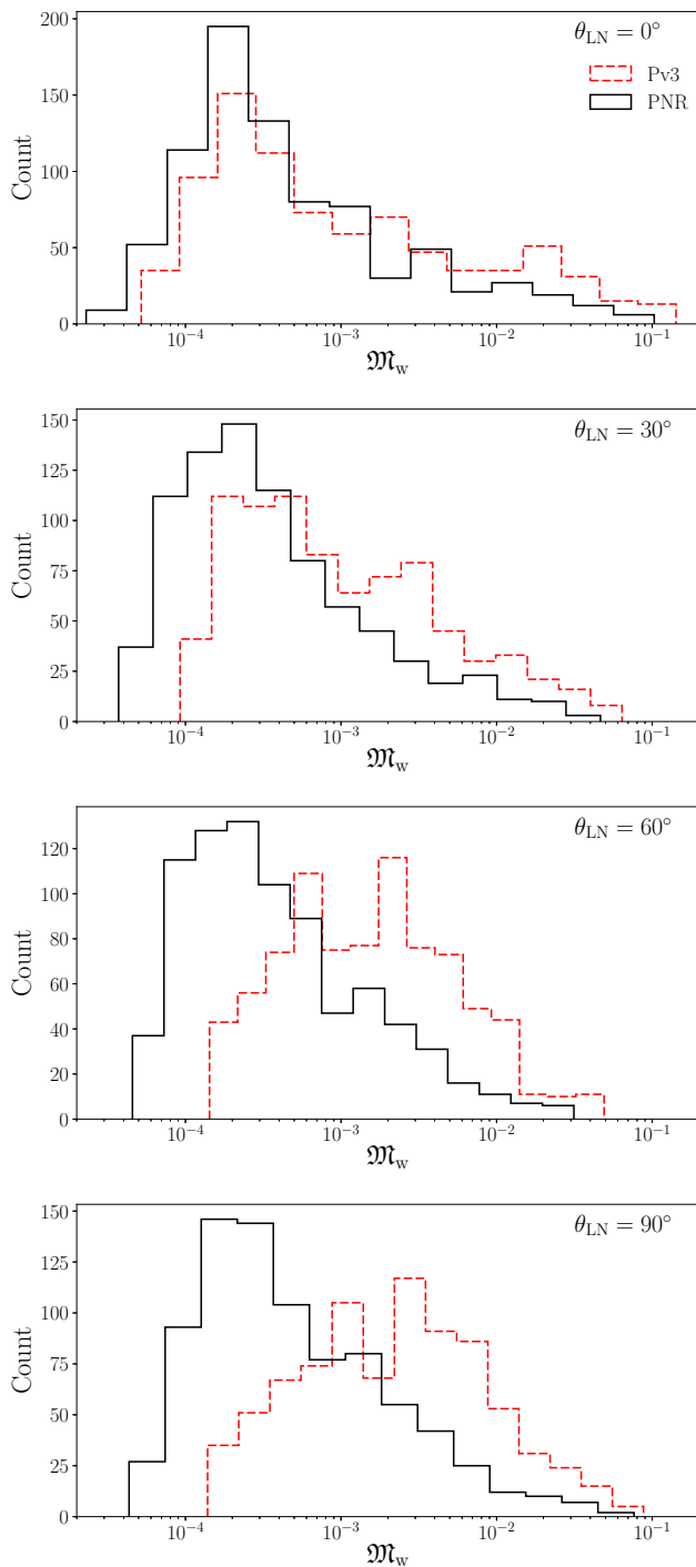
FIG. 21. Histograms of the SNR-weighted mismatches between the NR waveforms listed in Tables I-II and the waveform models PHENOMPv3 and PHENOPNR. Each subplot contains the SNR-weighted mismatches for all total masses separated by inclination descending as \theta_{LN} \in [0^\circ, 30^\circ, 60^\circ, 90^\circ] . The mismatches for all total mass values listed in Sec. XI E are included at each inclination. The results for PHENOPNR are present in solid black while the results for PHENOMPv3 are given in dashed red.
