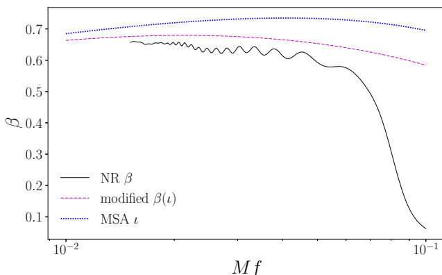
FIG. 5. Opening angles for the (q, \chi, \theta_{\text{LS}}) = (8, 0.8, 60^\circ) configuration. Solid black: the NR opening angle of the QA frame, \beta . Dotted blue: the PN opening angle of the orbital plane, \iota . Dashed magenta: Approximate QA angle \beta as a function of \iota ; see text for details.
