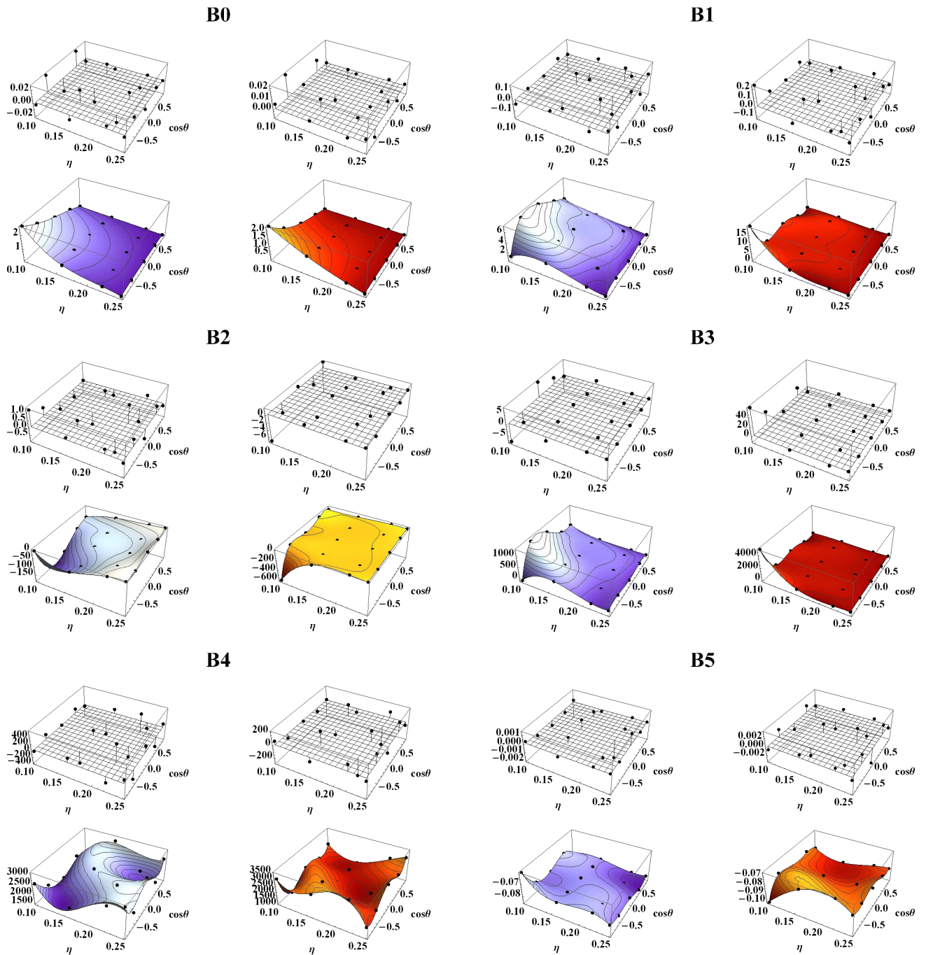
FIG. 28. Comparison of the fits for each of the co-efficients for the ansatz for \beta given in equation 49 with the co-efficients found from the data as described in Sec. VII. The fits are shown as two-dimensional surfaces covering the parameter space described by \eta and \cos\theta_{LS} . On the left in blue are the fits for the simulations with \chi = 0.4 and on the right in red are the fits for \chi = 0.8 . Above each of these surfaces are shown the residuals.
