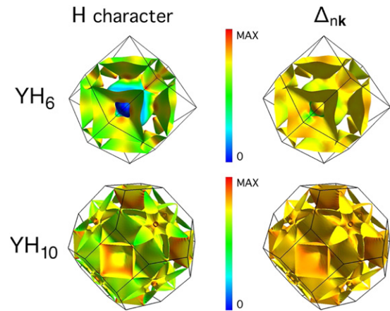
Figure 7. FSs of YH 6 (top row) and YH 10 (bottom row). In the left panels, the color scale spans the projection onto H states where blue corresponds to 0 and red to 1; in the right panels, it spans the values of the anisotropic gap function at 40 K, blue being 0 meV and red the maximum of 59 and 74 meV for YH 6 and YH 10 , respectively. Reprinted figure with permission from [35], Copyright (2019) by the American Physical Society.
