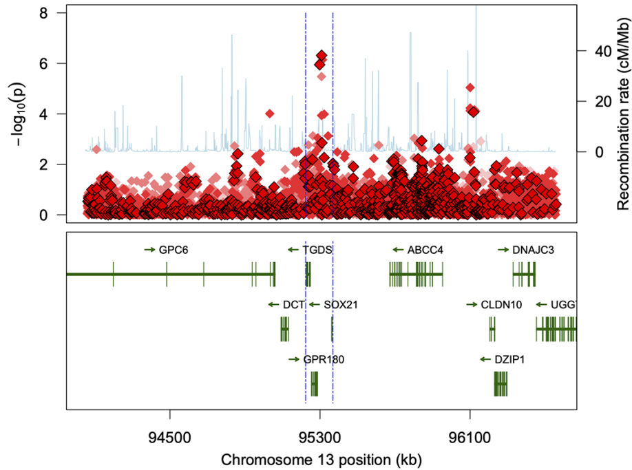
Figure 2. Manhattan diagram for the region surrounding rs9524583 (GRCh37). (Top) Association results for genotyped SNPs (red diamonds with black borders) and imputed SNPs (red diamonds, with saturation denoting imputation quality). Recombination rate is plotted with a solid blue line. (Bottom) Genes located in the region. Vertical rectangles indicate exons. (Both) Vertical blue dashed lines indicate the region identified by clustering, in which the critical variant is likely to lie.
