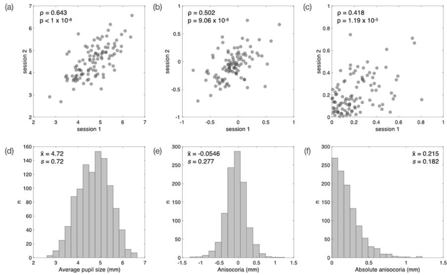
Figure 1. Test-retest reliabilities and distributions for average pupil size (a and d), signed anisocoria (b and e) and absolute anisocoria (c and f).
