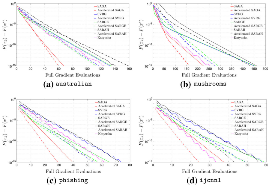
Fig. 1 Performance comparison for solving ridge regression among different algorithms
