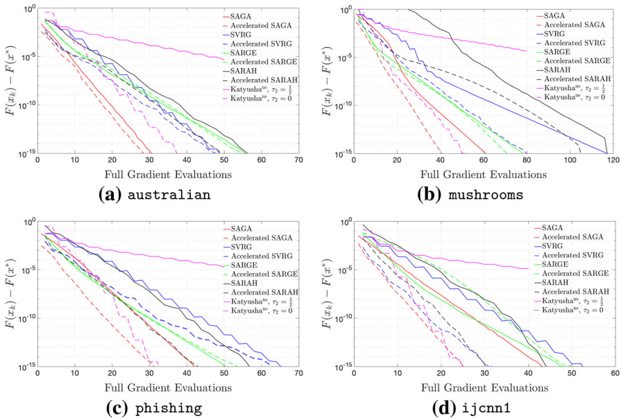
Fig. 2 Performance comparison for solving LASSO among different algorithms. In Katyusha, the negative momentum parameters \tau_2 = 0, \frac{1}{2} are not tuned
