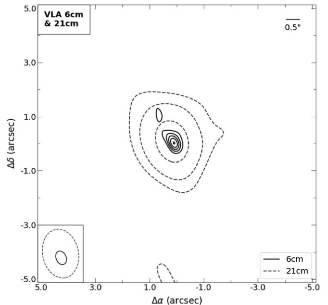
Figure 1. Contours of both the 21 and 6 cm VLA images. Contours for the 21 cm data are given on a logarithmic scale, -3\sigma , 3\sigma , 9\sigma , 27\sigma , \dots , where \sigma is the 21 cm rms noise. Contours for the 6 cm data are given on a linear scale, -5\sigma , 5\sigma , 9\sigma , 13\sigma , \dots , where \sigma is the 6 cm rms noise. The clean beams used to restore each of the images are given superimposed and to-scale in the bottom left-hand corner. The image shows the initial detection of an unresolved radio source within J132323.
