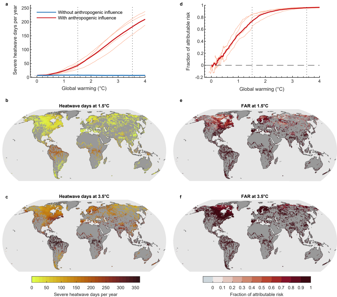
Figure 3. Global change in the occurrence of severe lake heatwaves and the role of anthropogenic forcing. Shown are (a) the globally averaged occurrence of severe lake heatwave days under different levels of global warming; (b) and (c) the spatial patterns in the number of severe heatwave days under a global warming of 1.5 and 3.5°C; (d) the fraction of attributable risk (FAR) under different global warming levels; and (e), (f) the spatial patterns in FAR under a global warming of 1.5 and 3.5°C. The thick lines in panels (a) and (d) illustrate the mean across the lake-climate model ensemble and the thin lines represent the global averages from the individual models. The time series are smoothed with a 30-year running mean. Panels (b, c, e, and f) show the averages from the multi-model ensemble over the 15-year period centered around the year when the respective global warming level is reached. Global warming levels are calculated as the globally averaged surface air temperature anomalies relative to the 1861 to 1900 base period. The vertical dashed lines in (a) and (d) illustrate a global warming of 1.5 and 3.5°C. The horizontal dashed line in panel (d) illustrates an FAR of 0.
