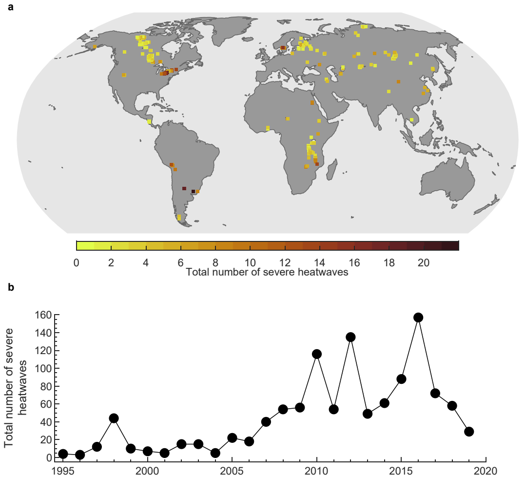
Figure 1. The global occurrence of severe lake heatwaves since 1995. Shown in panel (a) is the total number of severe heatwave events observed in each studied lake from 1995 to 2019. In panel (b), we show the total number of severe lake heatwaves observed across the studied lakes each year during the study period.
