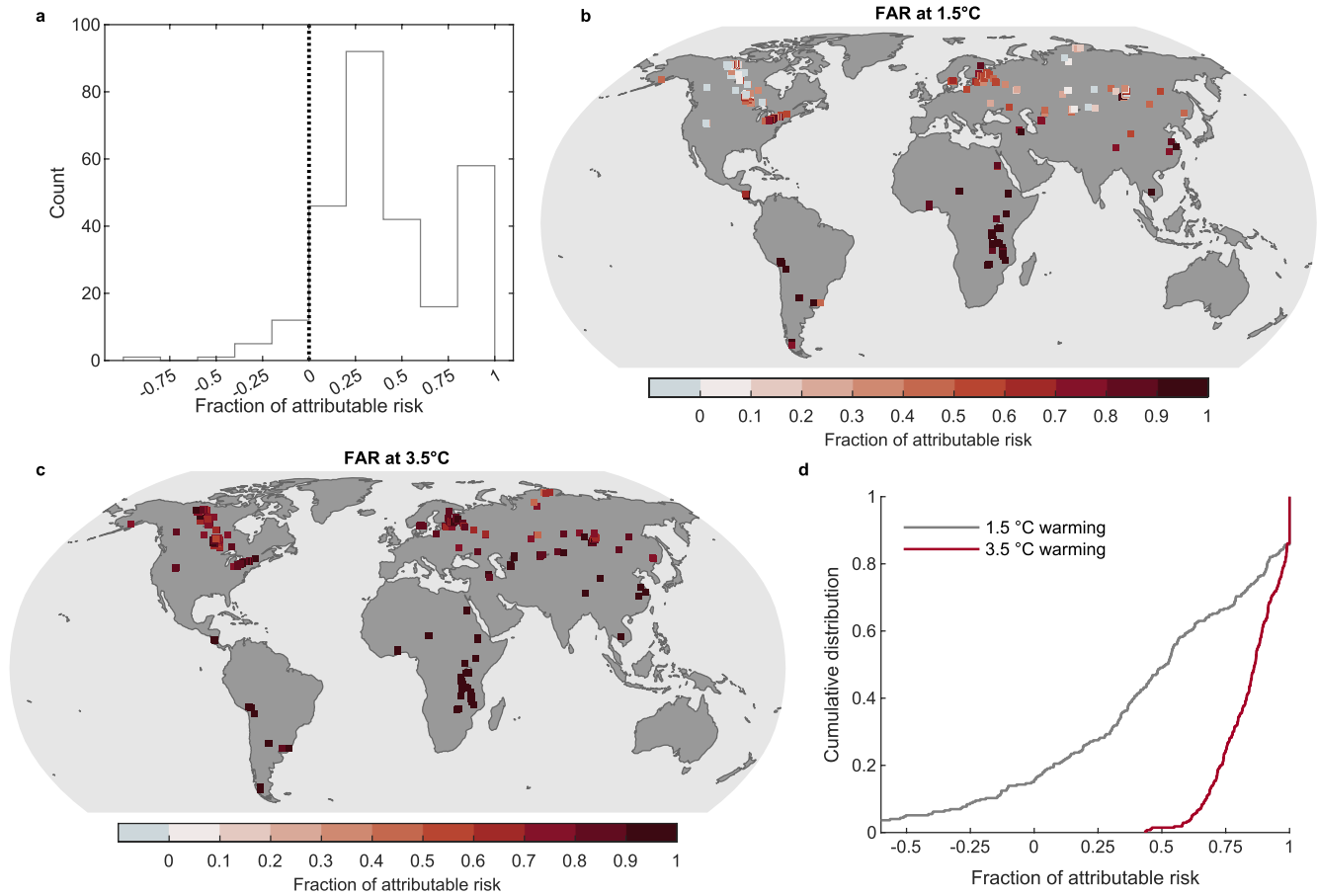
Figure 2. Anthropogenic contribution to severe lake heatwaves observed since 1995. Shown are (a) the fraction of attributable risk (FAR) of the observed severe lake heatwaves identified from satellite observations and model simulations from the historical to contemporary period with the vertical dashed line representing an FAR = 0; (b and c) the FAR of severe heatwaves under a global warming of 1.5 and 3.5°C; (d) the cumulative distribution of FAR under 1.5 and 3.5°C, as shown in panels (b and c). Results are shown for the average across the multi-model ensemble. The FAR values quoted under 1.5 and 3.5°C are calculated during a 15-year period centered around the year when the respective global warming level is reached. Global warming levels are calculated as the globally averaged surface air temperature anomalies relative to the 1861 to 1900 base period.
