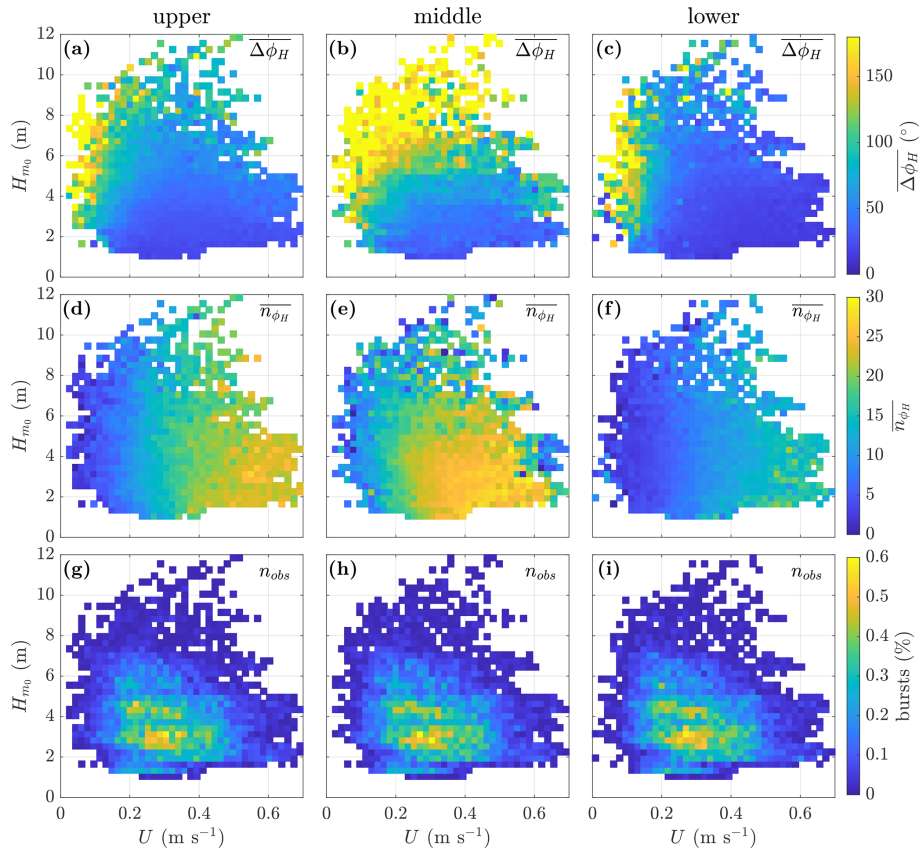
Figure 5. Mean heading oscillation range \overline{\Delta\phi_H} ( ^\circ ) (a–c), mean heading oscillations per burst \overline{n_{\phi_H}} (d–f), and percentage of bursts (g–i) for bursts aggregated by current speed, U ( \text{m s}^{-1} ), and significant wave height, H_{m_0} (m), for the deployment period 22 November 2014 to 4 April 2015, with aggregation bin \delta U = 0.0175 \text{ m s}^{-1} and \delta H_{m_0} = 0.3 \text{ m} . The instrument mooring position is shown above each column.
