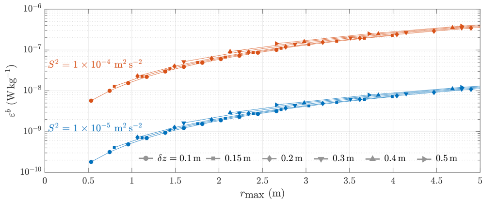
Figure 2. Potential bias due to shear using the standard method regression when none of the non-turbulent velocity differences between bins due to shear are removed ( \varepsilon^b ), evaluated for selected levels of shear S^2 , bin sizes \delta z , and maximum separation distance used for the regression r_{\max} .
