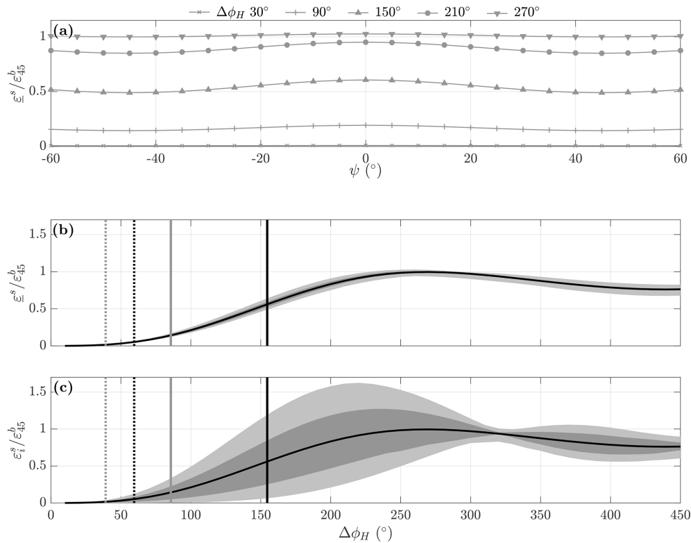
Figure 8. Normalised residual bias for heading oscillation scenarios. (a) Variation of beam-averaged normalised residual bias, \underline{\varepsilon}^s / \varepsilon_{45}^b , with initial heading offset angle to the background flow, \psi , for selected heading oscillation ranges \Delta\phi_H and fixed heading oscillation period t_{\phi_H} = 30 s. (a) Mean \underline{\varepsilon}^s / \varepsilon_{45}^b (black line), with 25 % to 75 % range (dark grey shading) and 5 % to 95 % range (light grey shading) for scenarios aggregated by \Delta\phi_H . (c) Mean and ranges for the maximum normalised beam residual bias \varepsilon_i^s / \varepsilon_{45}^b as in panel (b) . The vertical lines in panels (b) and (c) are the deployment 4 median (dotted line) and 90th percentile (solid line) \Delta\phi_H values for the upper (grey) and middle (black) instruments from the observations described in Sect. 3.
