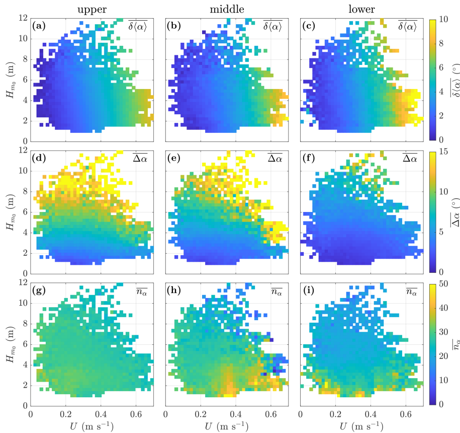
Figure 6. Mean tilt \overline{\delta\langle\alpha\rangle} (°) (a–c), mean tilt range \overline{\Delta\alpha} (°) (d–f), and mean tilt oscillations per burst \overline{n_{\phi H}} (g–i) for bursts aggregated by current speed, U ( \text{m s}^{-1} ), and significant wave height, H_{m0} (m), for the deployment period 22 November 2014 to 4 April 2015, with aggregation bin \delta U = 0.0175 \text{ m s}^{-1} and \delta H_{m0} = 0.3 \text{ m} . The instrument mooring position is shown above each column.
