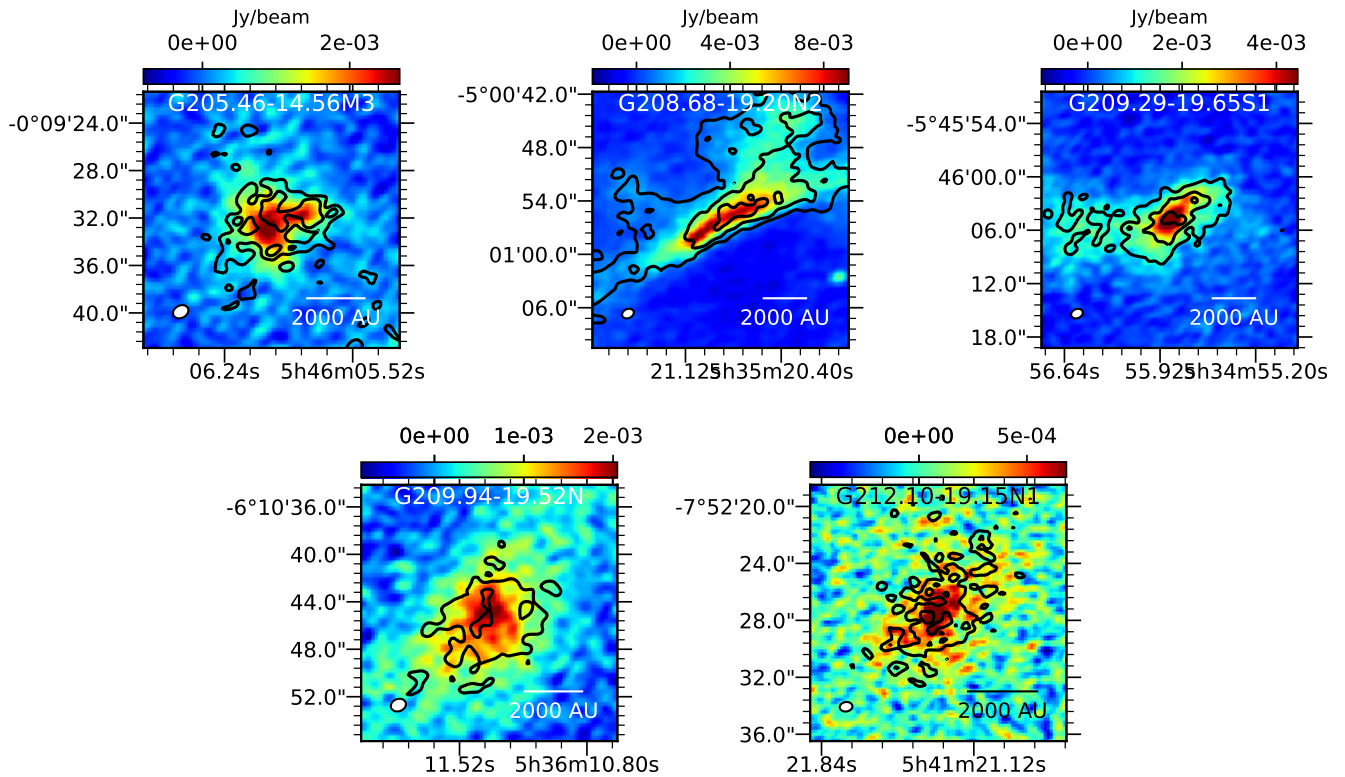
Figure 3. Integrated \text{N}_2\text{D}^+ emission in contours overlplotted on the ALMA ACA+TM2 dust continuum map. The contours are 3\sigma , 5\sigma , 7\sigma ..., where \sigma (rms)=20 and 17 mJy/beam \text{km s}^{-1} for G205.46-14.56M3 and G212.10-19.15N1 respectively. For G208.68-19.20N2, G209.29-19.65S1, G209.94-19.52N the rms ( \sigma )=32,20,21 mJy/beam \text{km s}^{-1} , respectively and contours are 5,10,15 \sigma .
