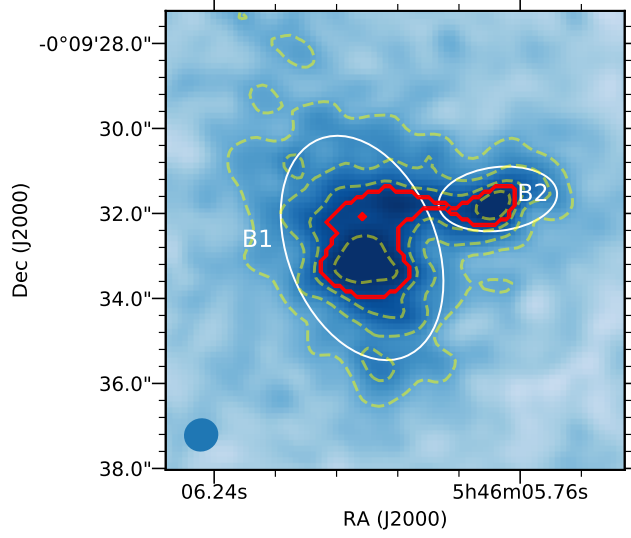
Figure A1. The red-contours show the condensations/blobs as identified using dendrogram analysis. White ellipses corresponds to FWHM size of the two component Gaussian fitting of the condensations B1 and B2. Dotted contours corresponds to 1.3mm dust continuum at 0.8'' resolution with the levels 4,7,10,13 \sigma where the rms noise is given by \sigma = 0.1 mJy/beam.
