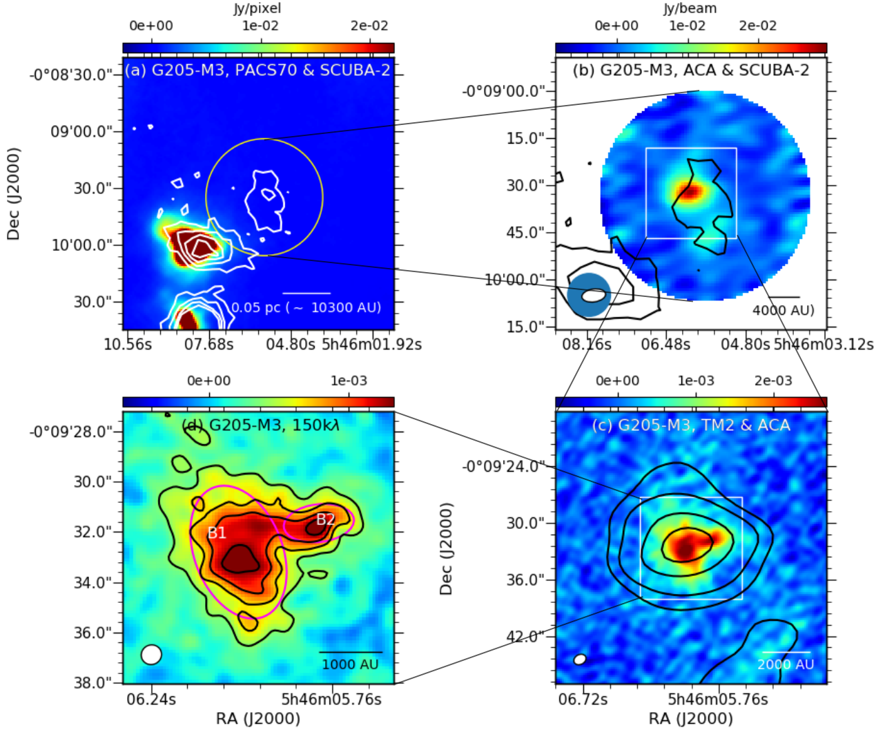
Figure 2. The structure of G205.46-14.56M3 as revealed at different wavelengths and scales. Panel (a) shows 1.3 mm continuum observed by SCUBA-2 in contours: 0.3, 0.5, 0.7, 0.9 \times peak (where peak = 671.4 mJy/beam corresponds to the peak flux of closest protostellar core) overplotted on the 70 \mu\text{m} mid-infrared image taken by Herschel PACS. Panel (b) shows the SCUBA-2 850 \mu\text{m} continuum in contours ( 6\sigma , \sigma = 38 \text{ mJy/beam} ) and the ACA 1.3 mm continuum map in color. Both beams are shown in left bottom corner. Panel (c) shows the highly dense central region as revealed by the ALMA ACA+TM2 dust continuum map (synthesized beam \sim 1.2'' ). Plotted in contours are the ACA continuum with levels 3.5, 10, 15\sigma, \dots , where \sigma = 1.6 \text{ mJy/beam} . Panel (d) zooms toward the central region at a higher resolution (synthesized beam 0.8'' ) where the substructures (B1 & B2) are visible. The contours are at 4, 6, 10 and 13 \sigma levels where \sigma = 0.1 \text{ mJy/beam} . The ellipses correspond to the FWHM sizes inferred from the two-component Gaussian fitting.
