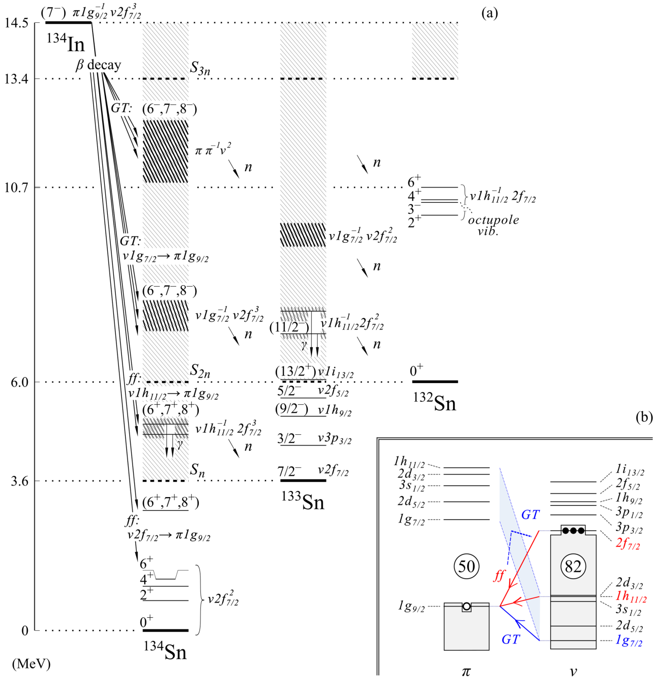
FIG. 11. (a) Schematic \beta -decay scheme of ^{134}\text{In} showing Gamow-Teller (GT) and first-forbidden ( ff ) transitions that populate neutron-unbound (gray striped areas) and bound states in the daughter nuclei. The expected excitation energies of unobserved states having core-excited configurations are indicated by black striped areas. Neutron-unbound states for which decay via \gamma -ray emission was observed are indicated. (b) Schematic representation of proton ( \pi ) and neutron ( \nu ) orbitals relevant for the \beta decay of ^{134}\text{In} [61]. The ground-state configuration of the parent nucleus is schematically represented by circles indicating the location of valence neutrons (full circles) and proton hole (open circle) relative to the ^{132}\text{Sn} core.
