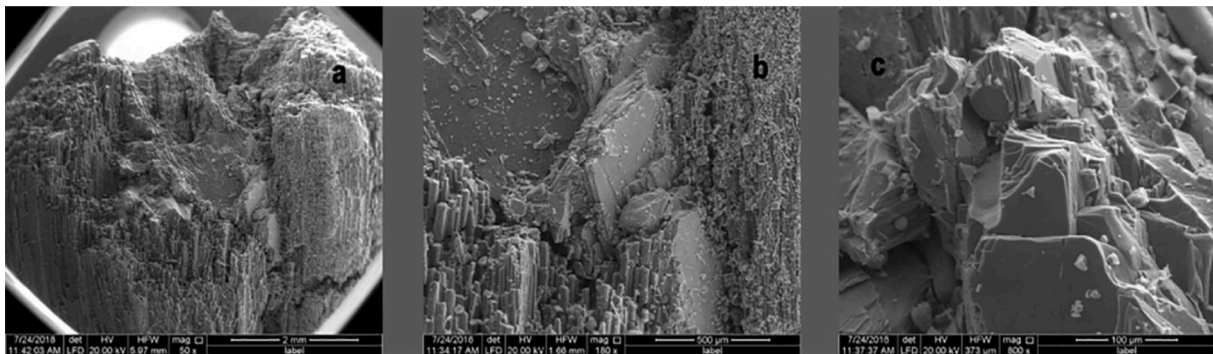
Fig. 6. Various magnifications of SEM images showing a wooden fragment presenting vivianite encrustations.
