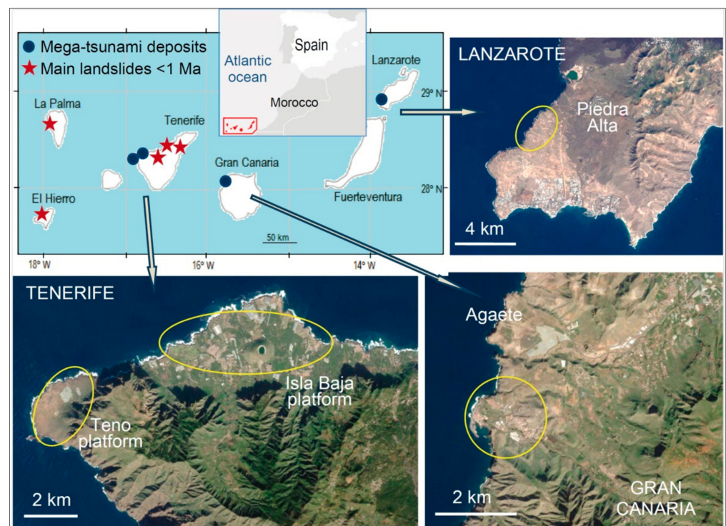
Figure 1. Location of the tsunami deposits and main recent (<1 Ma) megalandslides in Canary Islands. Satellite images with the location of the tsunami deposits at Teno and Isla Baja platforms, Tenerife; Piedra Alta, Lanzarote; and Agaete, Gran Canaria. Google Earth images.
