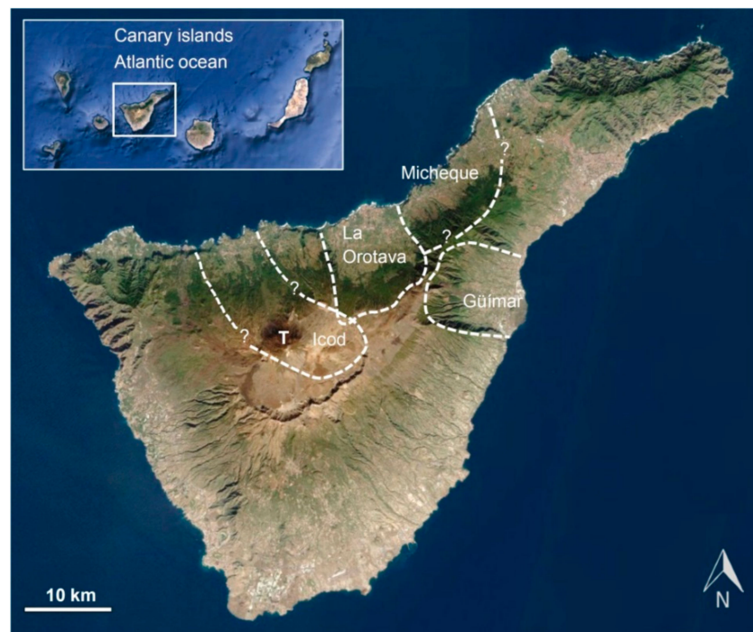
Figure 13. Schematic representation of the most recent landslides in Tenerife: Icod, La Orotava, Guímar, and Micheque or Acentejo, the latter without morphological features on surface. T: Teide volcano (3715 m). Limits of Micheque landslide from [76]. Basemap: GRAFCAN.
