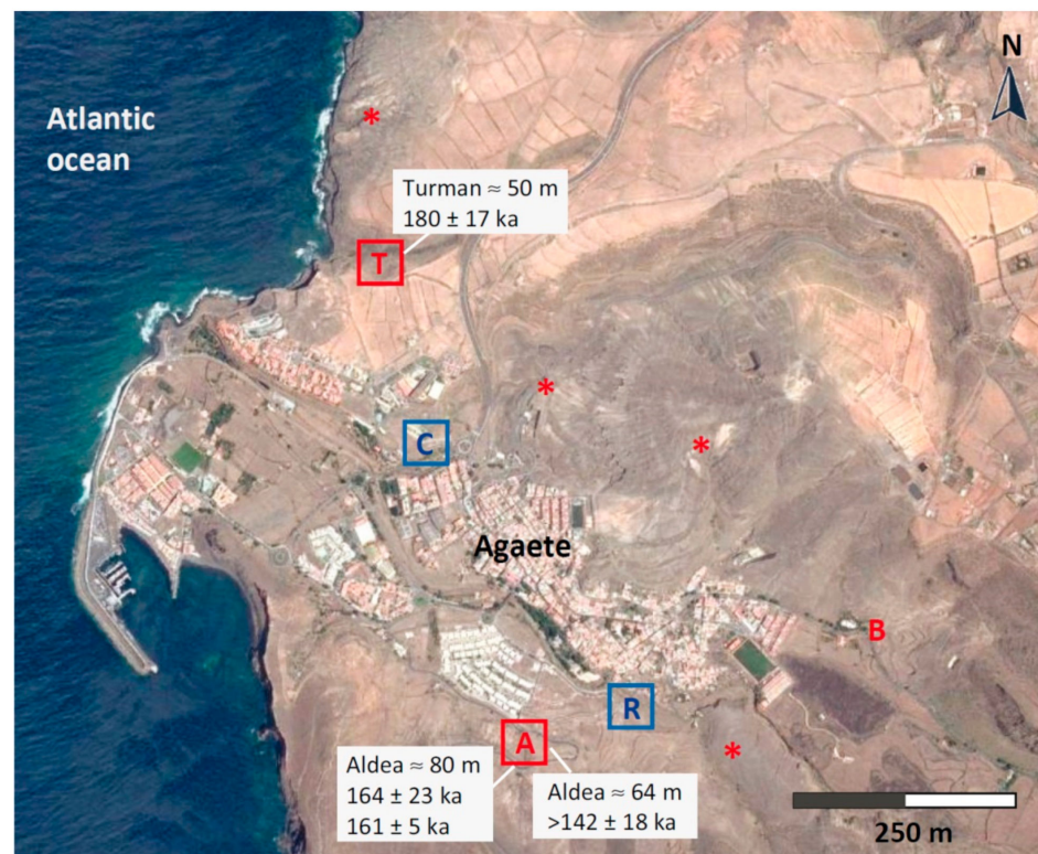
Figure 10. Location of the outcrops of tsunamigenic conglomerates in the area of Agaete (red stars and letters), first described in [8]. Outcrops cited in the text: Llanos de Turman (T); Berrazales (B); La Aldea (A). New outcrops referred in the text (blue): El Cementerio (C) and La Ruina (R). Ages obtained in this study for La Aldea and Llanos de Turman sites are included. Image from Google Earth.
