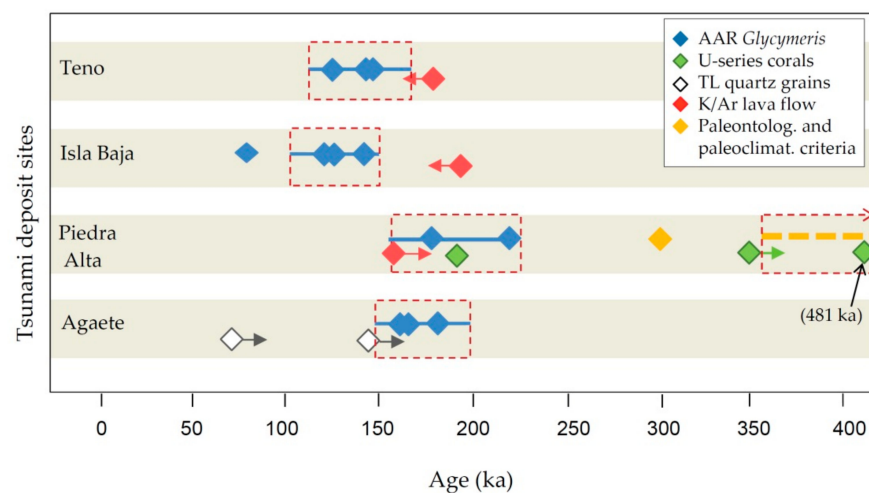
Figure 12. Plot of the age determinations for the tsunami deposits in Tenerife, Lanzarote, and Gran Canaria. K/Ar and paleo-criteria ages from the literature. The dashed red rectangles indicate the most probable ages for the deposits. For Piedra Alta, two alternative age intervals are indicated, although we favor the younger age.
