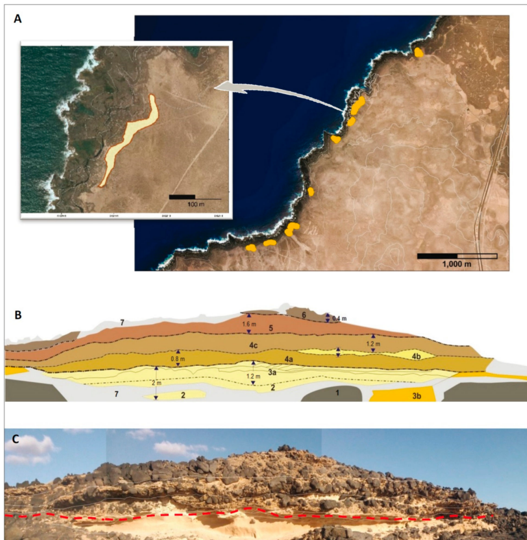
Figure 8. (A) Tsunami deposits outcrops scattered along the SW coast of Lanzarote, and location of the main Piedra Alta outcrop. PNOA and Google images. (B) Geological cross section of the Piedra Alta deposits in the coastal cliff, at ~20 m a.s.l. 1: underlying lava flow; 2,3: Aeolian sand (paleo dune) and clayey paleosol containing abundant terrestrial fossil fauna, 2 m max.; 4,5,6: tsunami conglomerates showing different layers with erosive contact, cemented sand matrix and basalt angular blocks, terrestrial and marine fossils, 4 m max.; 7: current sandy soil. (C) Annotated photograph of the outcrop; length: 30 m (the red line marks the base of the tsunami deposit).
