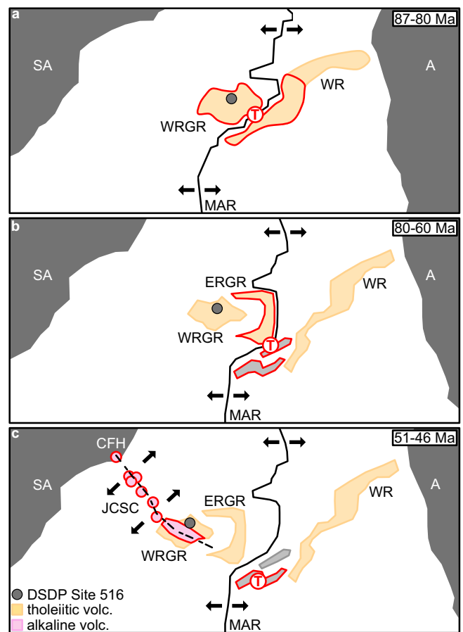
Fig. 7 Schematic sketch illustrating the geochemical and tectonic evolution of the Rio Grande Rise and Jean Charcot Seamount Chain (JCSC).
