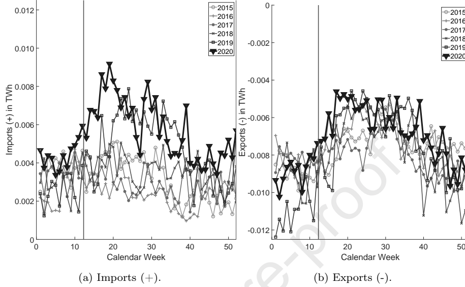
Figure 2: Profile for commercial imports and exports of DE-(AT)-LU for the years 2015 to 2020. The vertical lines represent the start of our period of interest. Own illustration, data from [50].
