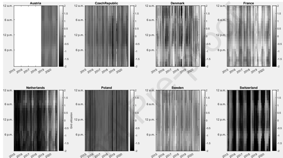
Figure 13: Heatmaps for the utilization of Germany's interconnection capacities from 2015 to 2020. Own illustration, data from [53, 52].
