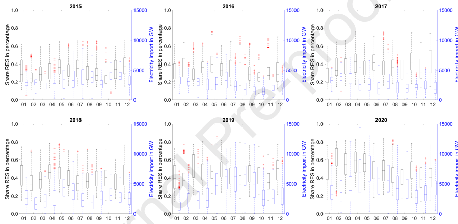
Figure 8: Monthly German share of RES and cumulative physical flow imports. Own illustration, data from [53, 52].
