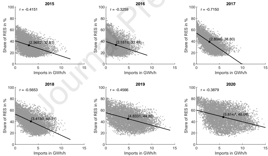
Figure 6: Cumulative commercial exchange imports and the corresponding share of RES of DE-(AT)-LU for the years 2015 to 2020. Own illustration, data from [50, 52].
