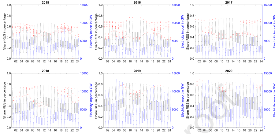
Figure 9: Daily German share of RES and cumulative physical flow imports. Own illustration, data from [53, 52].
