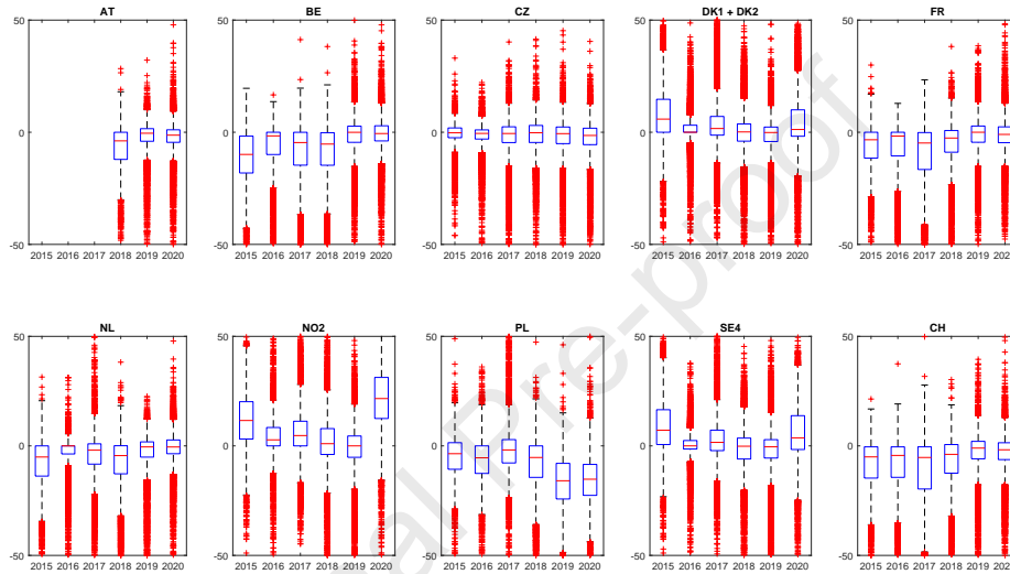
Figure 3: Differences in electricity prices on the Day-Ahead market between Germany and its neighboring bidding zones for the years from 2015 to 2020. Own illustration, data from [50].
