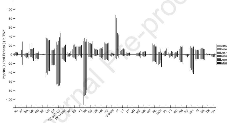
Figure 1: Cumulative commercial imports (+) and exports (-) of 38 European bidding zones for the years 2015 to 2020. Own illustration, data from [50].
