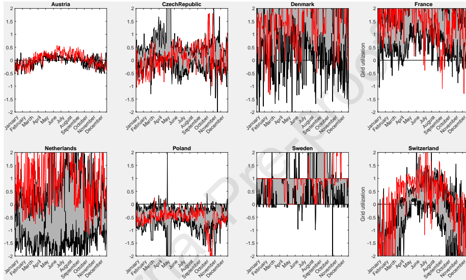
Figure 14: Daily maximum of interconnection capacities utilization of Germany from 2015 to 2020. Own illustration, data from [52, 53].
