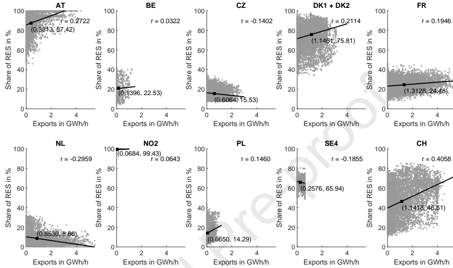
Figure 4: Cumulative commercial exports of its neighboring countries to Germany and the corresponding share of RES in the corresponding country Own illustration, data from [50, 52].
