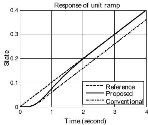
FIGURE 2. Integral state feedback for ramp input reference.
