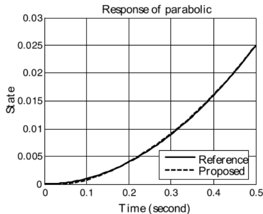
FIGURE 9. System response of parabolic input reference.
