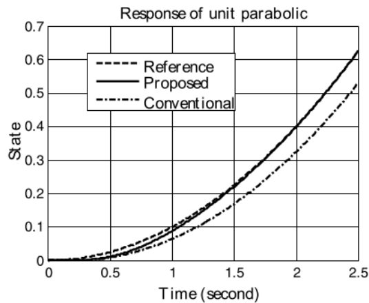
FIGURE 3. Integral state feedback for parabolic input reference.
