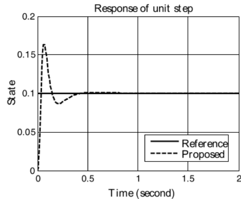
FIGURE 7. System response of step input reference.
