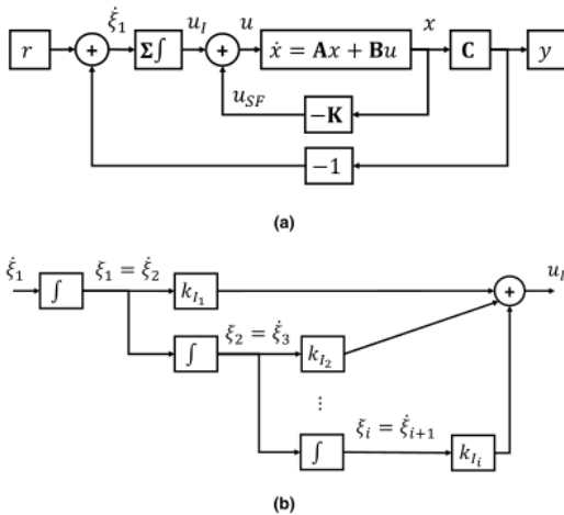
FIGURE 1. Integral state feedback.
