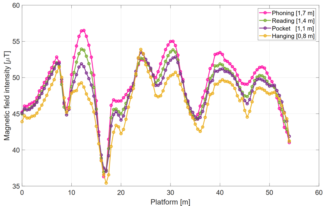
Figure 6: Magnetic intensity map of the norm of the three-axis magnetometer for the four magnetometers attached to the wooden structure shown in Figure 2, measured at the platform of the Gauting suburban train station with a 0.5 m spacing grid.
