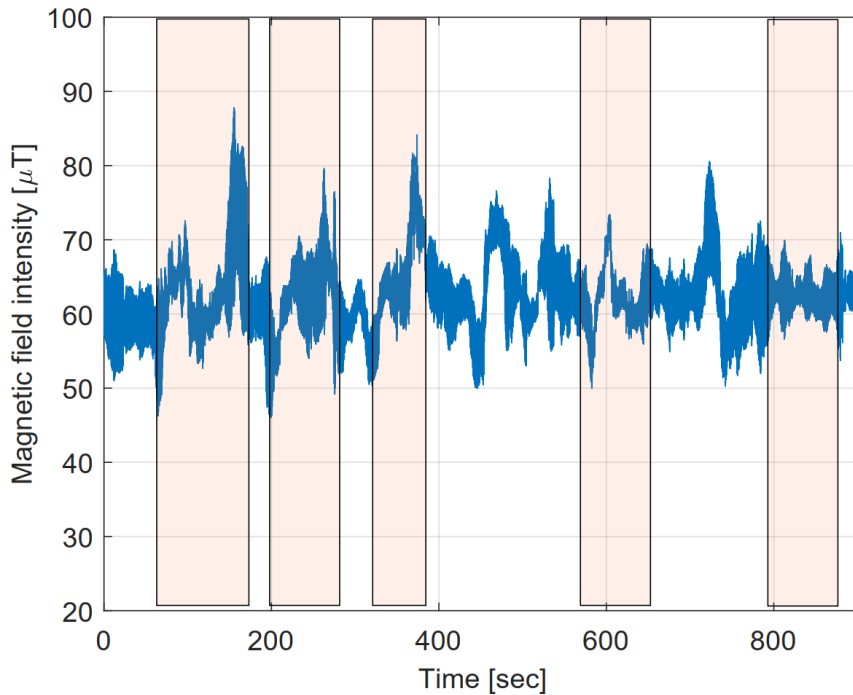
Figure 4: Norm of the three-axis magnetometer during static measurements at the platform of the Marienplatz suburban train station. The orange-shadowed areas indicate the train entering, staying and leaving the station.
