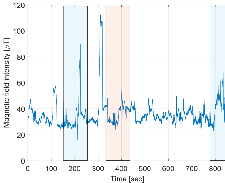
Figure 3: Norm of the three-axis magnetometer during static measurements at the platform of the Holzapfelkreuth subway station. The trains entering, staying and leaving the station have been marked with shadowed-areas: orange for the trains circulating on the main track and blue for the trains circulating on the adjacent track.
