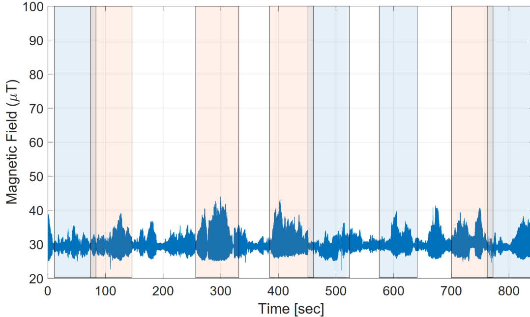
Figure 5: Norm of the three-axis magnetometer during static measurements at the platform of the Rosenheimer Platz suburban train station. The trains entering, staying and leaving the station have been marked with shadowed-areas: orange for the trains circulating on the main track and blue for the trains circulating on the adjacent track.
