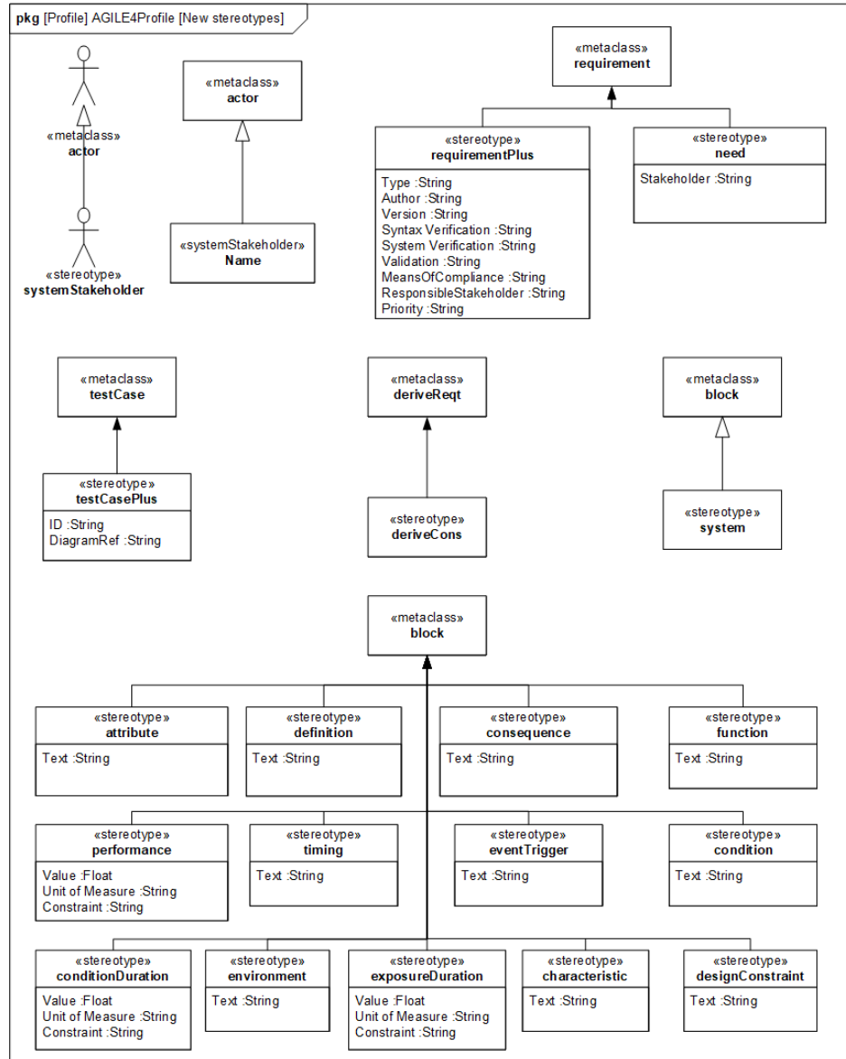
Figure 17 SysML Package Diagram representing the new stereotypes for the modeling of stakeholders, needs and requirements introduced with the new AGILE4Profile .
