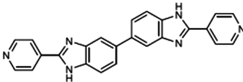
Figure 2 Chemical structure of ridinilazole [2,2'-bis(4-pyridyl) 3H,3'-H5,5-benzimidazole] (Weiss et al. 2014)
