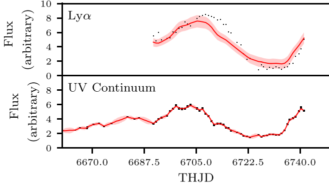
Figure 10. Same as Figure 1, but for the Ly \alpha BLR models. The residuals at 1216 Å are likely due to geocoronal Ly \alpha emission.
