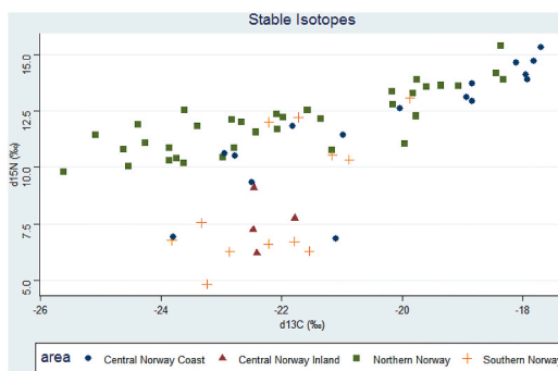
Fig. 2. Values of \delta^{13}\text{C} and \delta^{15}\text{N} in individual Eurasian eagle-owl ( Bubo bubo ) feathers collected in four areas across Norway. The individual stable isotope values are represented by points in different shapes and colors according to the areas where feathers were collected. For better understanding of the data, we have included here the four different areas collected, but because of small sample sizes Central Norway Inland and Central Norway Coast were pooled together for further statistical analysis. (For interpretation of the references to color in this figure legend, the reader is referred to the Web version of this article.)
