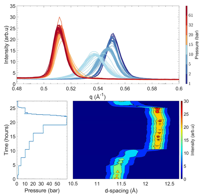
Figure 2. Evolution of the (002) Bragg reflection as a function of pressure at 26 °C for Ni-Hec 0.5 recorded via PXRD. The bottom left panel shows the measured pressure of CO 2 applied on the sample as a function of time, and the bottom right panel shows a contour plot in which the horizontal axis corresponds to d spacing ( d = 2\pi/q ). The vertical axis corresponds to time scaled by the same horizontal axis as for the pressure, and the color gradient represents the intensity. In the top panel, the evolution of the (002) Bragg reflection is plotted with colors indicating the approximate pressure.
