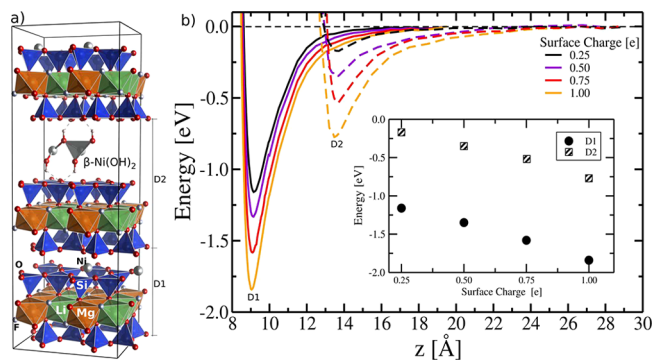
Figure 7. (a) Side view of the Hec molecular model highlighting the atomic configuration with a layer charge of 1.0 pfu (unit cell area of 9.2 Å × 5.3 Å) achieved by the substitution of two Mg atoms with Li atoms. (b) Energy curves for the dehydrated smectite (D 1 ) and for the β-Ni(OH) 2 island (D 2 ) in the interlayer space considering the role of the surface charges. The equilibrium position indicates the basal separation distance, while the depth of the potential well may be interpreted as the cohesion energy per unit cell. The basal d spacing can be obtained by the term (D 1 + D 2 )/2. The inset shows the energy minimum as a function of surface charge.
