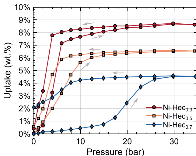
Figure 5. Comparison of the gravimetric adsorption capacity in dried Ni-Hec with layer charges Ni-Hec 0.3 , Ni-Hec 0.5 , and Ni-Hec 0.7 equilibrated for 4 h at each pressure step. The arrows show the sorption hysteresis with the increase or decrease in pressure.
