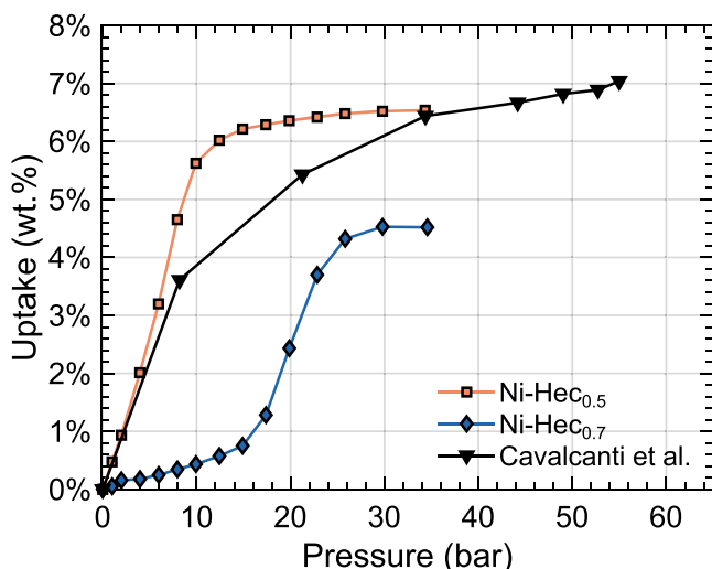
Figure 8. Comparison of the adsorption capacity of Ni-Hec 0.5 and Ni-Hec 0.7 compared with results on a Ni-Hec cation-exchanged from a commercial Corning sample. 15
