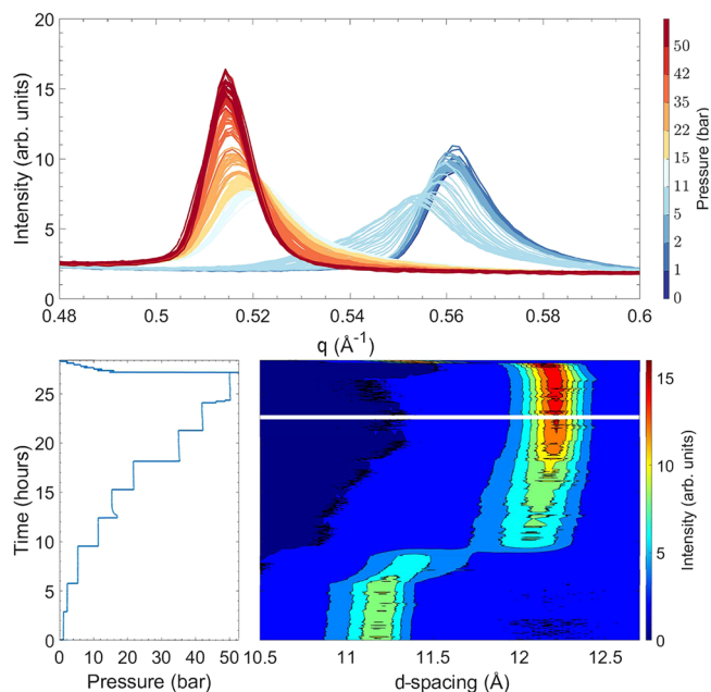
Figure 1. Evolution of the (001) Bragg reflection as a function of pressure at 26 °C for Ni-Hec 0.3 recorded via PXRD. The bottom left panel shows the measured pressure of CO 2 applied on the sample as a function of time, and the bottom right panel shows a contour plot in which the horizontal axis corresponds to the d spacing ( d = 2\pi/q ). The vertical axis corresponds to time scaled by the same horizontal axis as for the pressure, and the color gradient represents the intensity. In the top panel, the evolution of the (001) Bragg reflection is plotted with colors indicating the approximate pressure.
