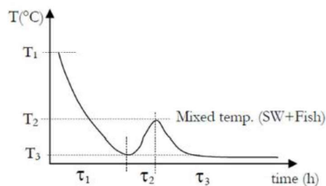
Figure 2: Characteristic chilling curves for a RSW system showing the prechilling and chilling process. Adapted from Thorsteinsson et al. (2003)
